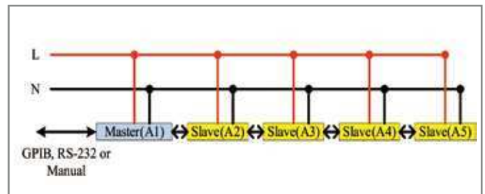
Figure 10: Parallel connection
