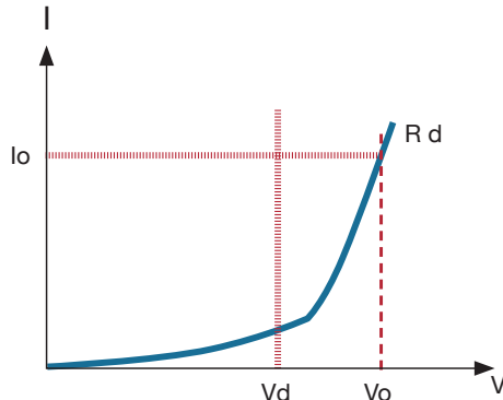
Figure - LED I-V Curve
