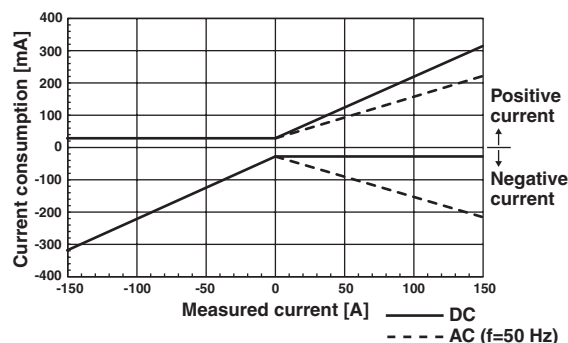
Current probe (701930)
