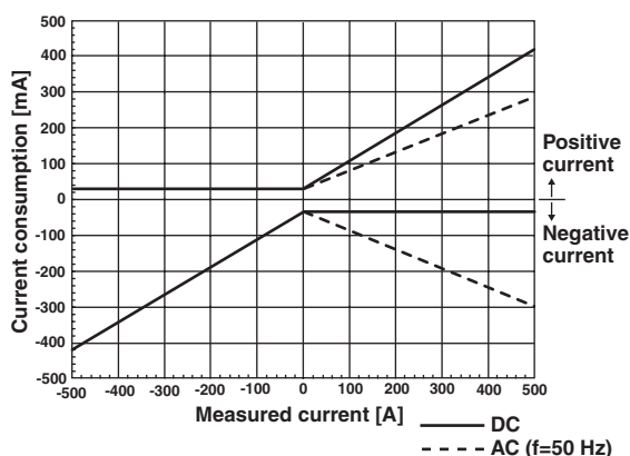
Current probe (701931)
