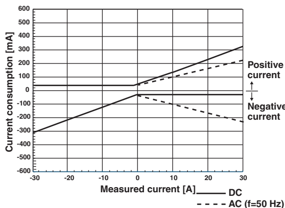
Current probe (701932)
