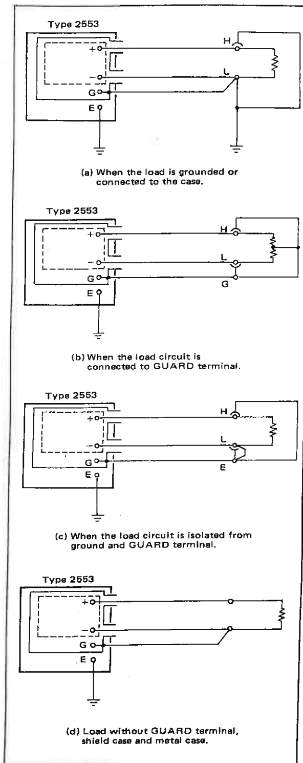
Figure 3-2. GUARD Terminal Connections.
