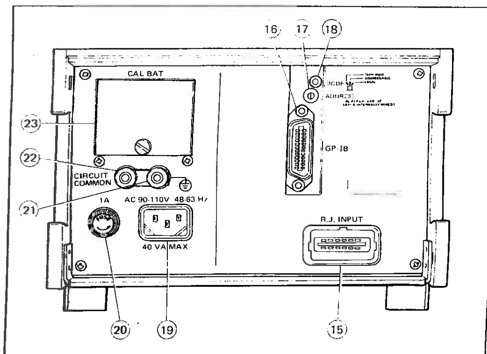
Figure 2-2. Rear Panel.
