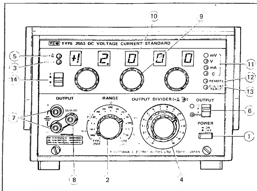
Figure 2-1. Front Panel.
