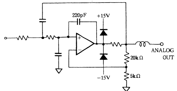
Figure 2-32 V, A and W Output Circuit
