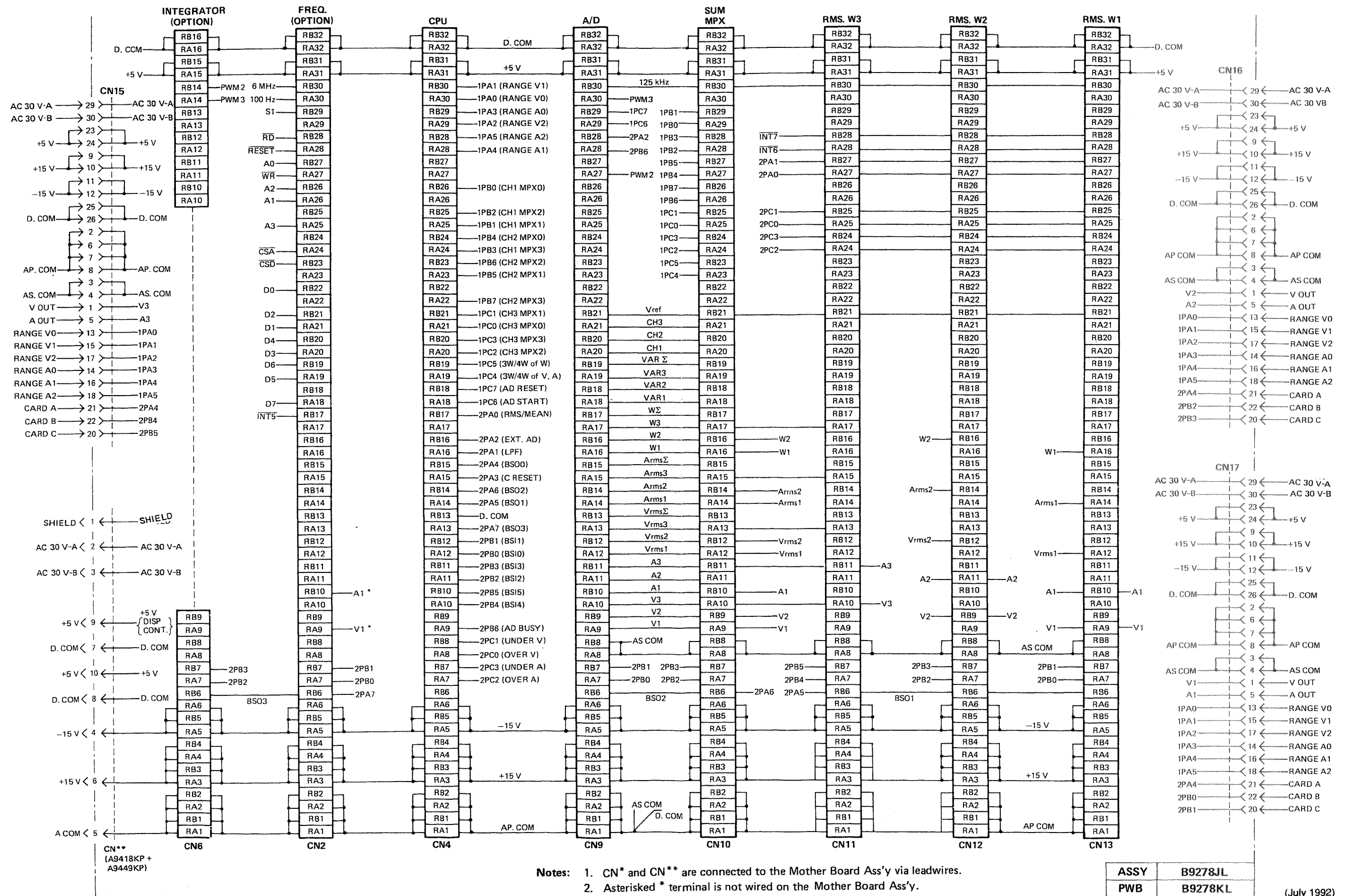
Figure 5-11b. Mother Board Ass'y: B9278JL Schematic Diagram (2/2).
