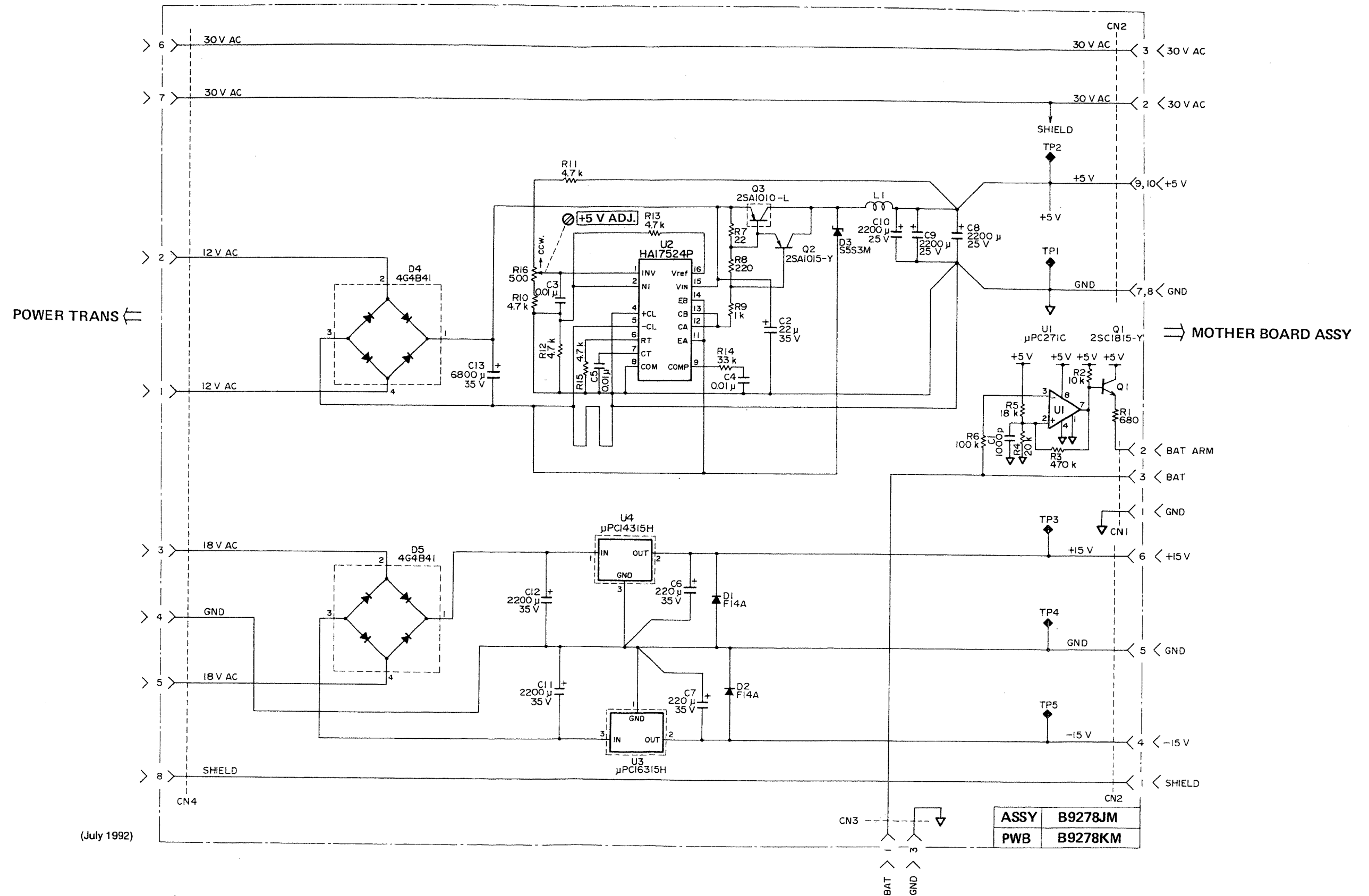
Figure 5-12a. Power Supply Board Ass'y (for Models 2533E32 and 2533E33): B9278JM Schematic Diagram.
