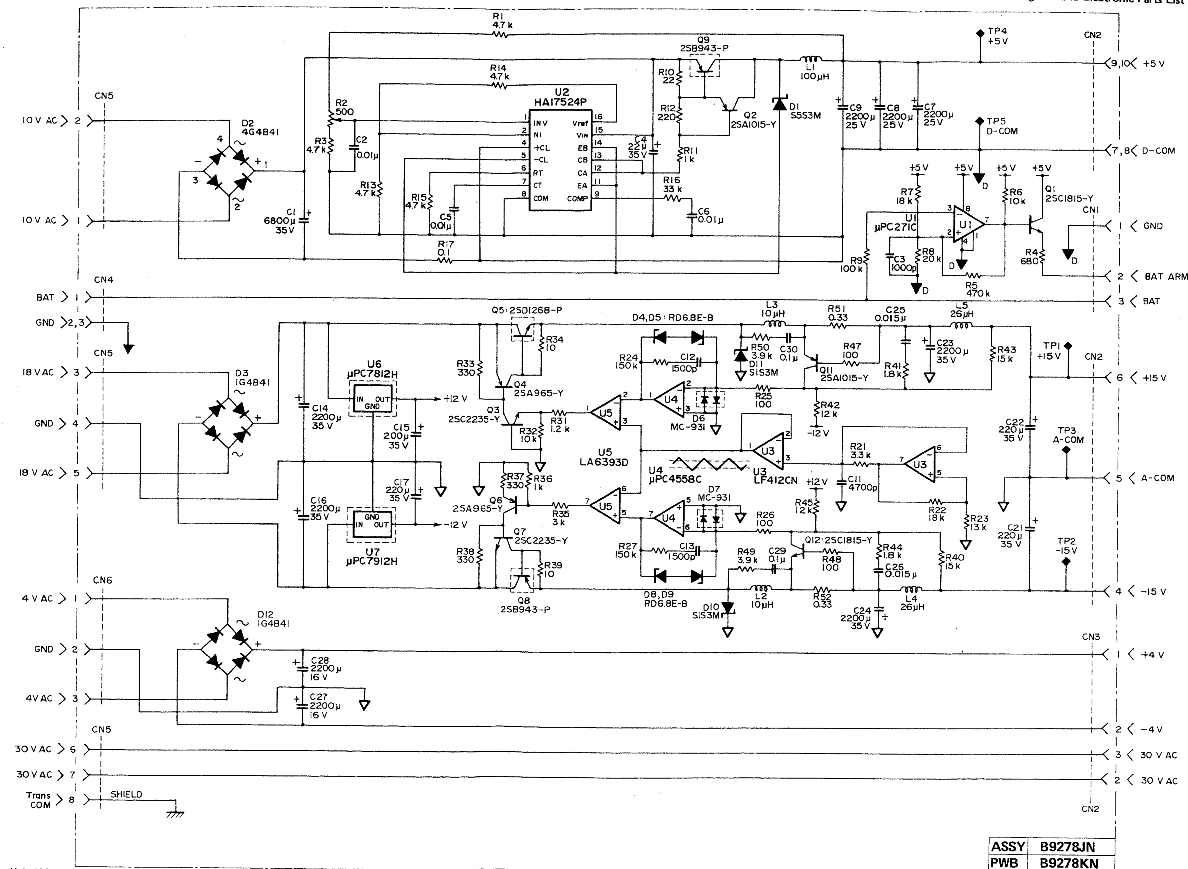
Figure 5-13a. Power Supply Board Ass'y (for Models 2533E42 and 2533E43): B9278JN Schematic Diagram.
