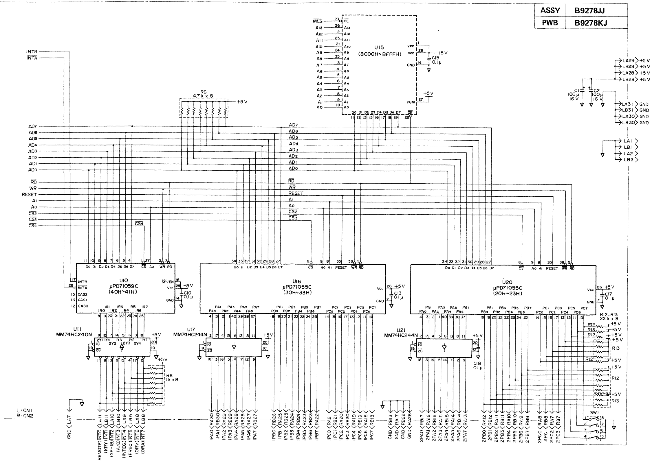
Figure 5-9b. CPU Board Ass'y: B9278JJ Schematic Diagram (2/2).
