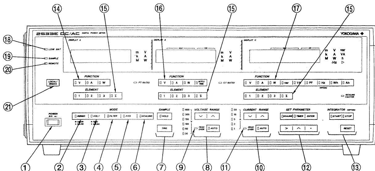
Figure 1-1. Front Panel
