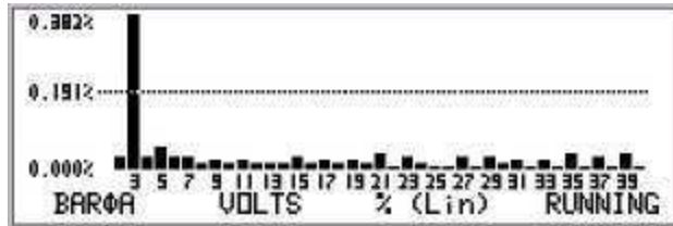
Figure 45. Harmonics Bargraph \phi A , VOLTS % Lin display
