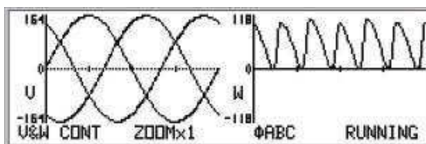
Figure 59. Waveforms V&W CONT \Sigma\phi ABC display
