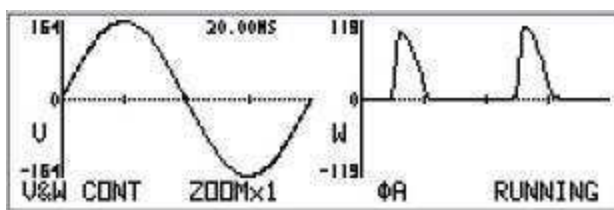
Figure 58. Waveforms V&W CONT \phi A display
