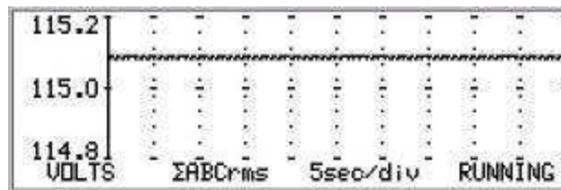
Figure 61. History VOLTS \Sigma\phi ABC RMS display
