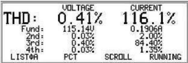
Figure 51. Harmonics List \phi A , PERCENTAGE display
