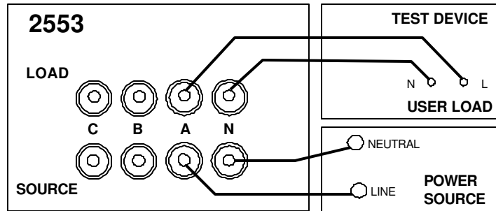
Figure 13. 1 \phi 2-Wire Connections diagram
