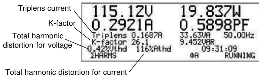
Figure 40. Basics \Sigma HARMS \phi A display with callouts
