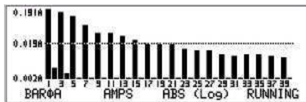
Figure 48. Harmonics Bargraph \phi A , AMPS ABS Log display
