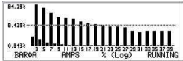
Figure 46. Harmonics Bargraph \phi A , AMPS % Log display
