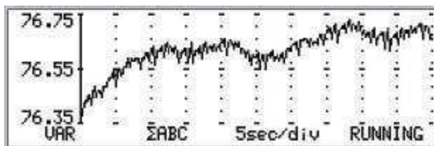
Figure 75. History VAR \Sigma\phi ABC display
