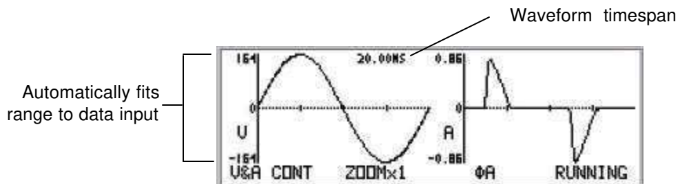
Figure 54. Waveforms V&A CONT \phi A display with callouts
