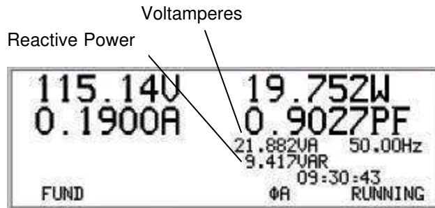
Figure 38. Basics FUND \phi A display with callouts
