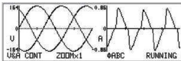
Figure 57. Waveforms V&A CONT \Sigma\phi ABC display
