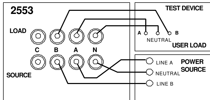
Figure 14. 1 \phi 3-Wire Connections diagram
