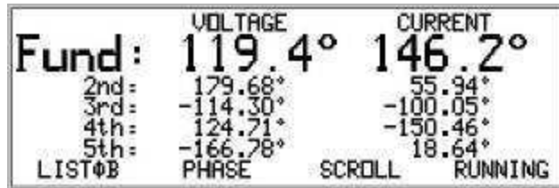
Figure 53. Harmonics List \phi B , PHASE display
