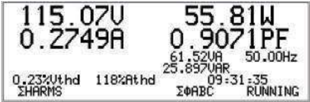
Figure 41. Basics \Sigma HARMS \Sigma\phi ABC display
