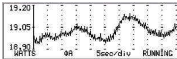
Figure 72. History WATTS \phi A display
