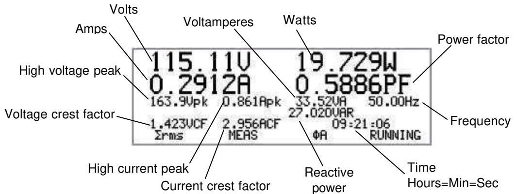
Figure 22. Basics \Sigma RMS MEAS \phi A display with callouts
