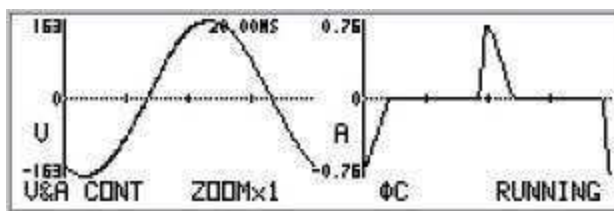
Figure 56. Waveforms V&A CONT \phi C display
