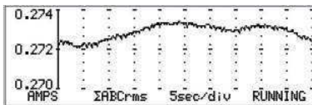
Figure 67. History AMPS \Sigma\phi ABC RMS display
