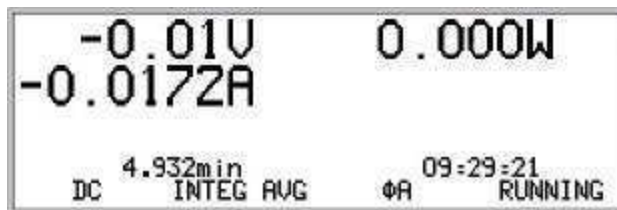
Figure 36. Basics DC INTEG AVG \phi A display
