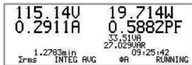
Figure 28. Basics \Sigma RMS INTEGR AVG \phi A display
