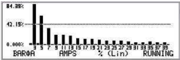
Figure 49. Harmonics Bargraph \phi A , AMPS % Lin display
