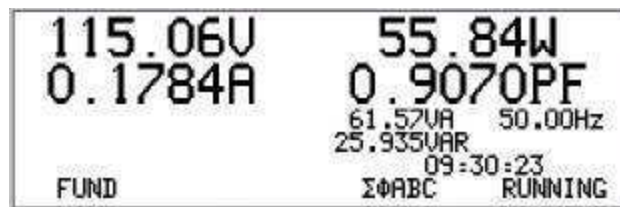
Figure 39. Basics FUND \Sigma\phi ABC display
