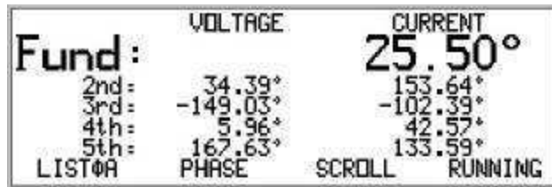
Figure 52. Harmonics List \phi A , PHASE display
