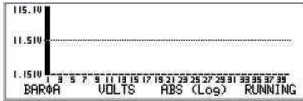
Figure 44. Harmonics Bargraph \phi A , VOLTS ABS Log display
