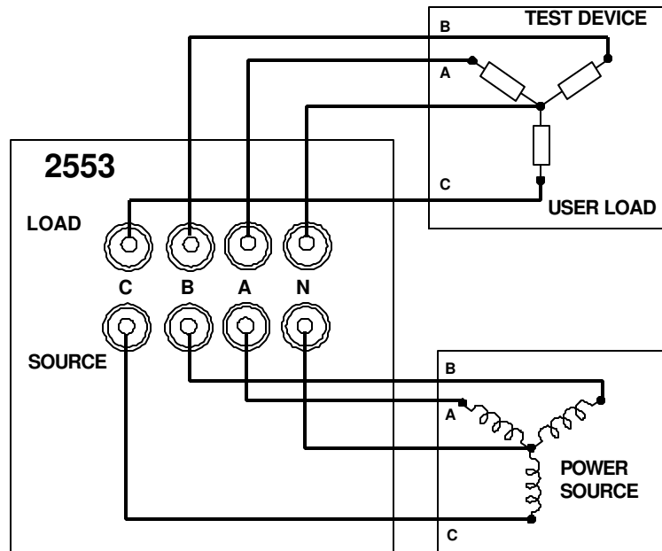
Figure 16. 3 \phi 4-Wire Connections diagram
