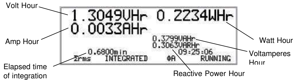
Figure 26. Basics \Sigma RMS INTEGRATED \phi A display with callouts
