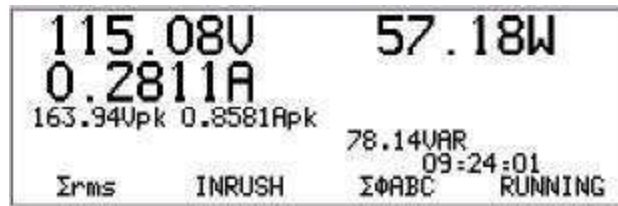
Figure 25. Basics \Sigma RMS INRUSH \Sigma\phi ABC display
