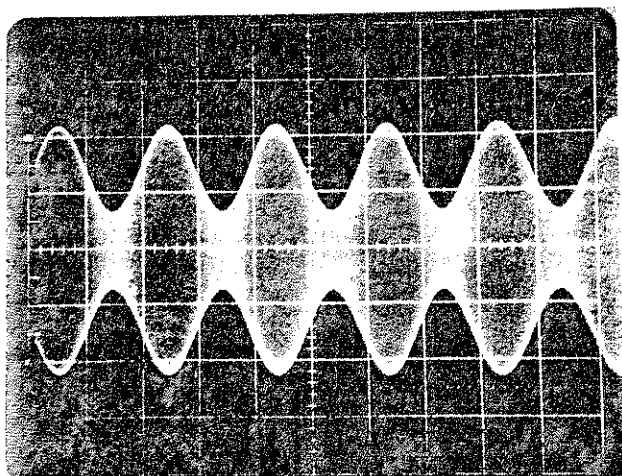
Figure 2-5. Amplitude Modulation
