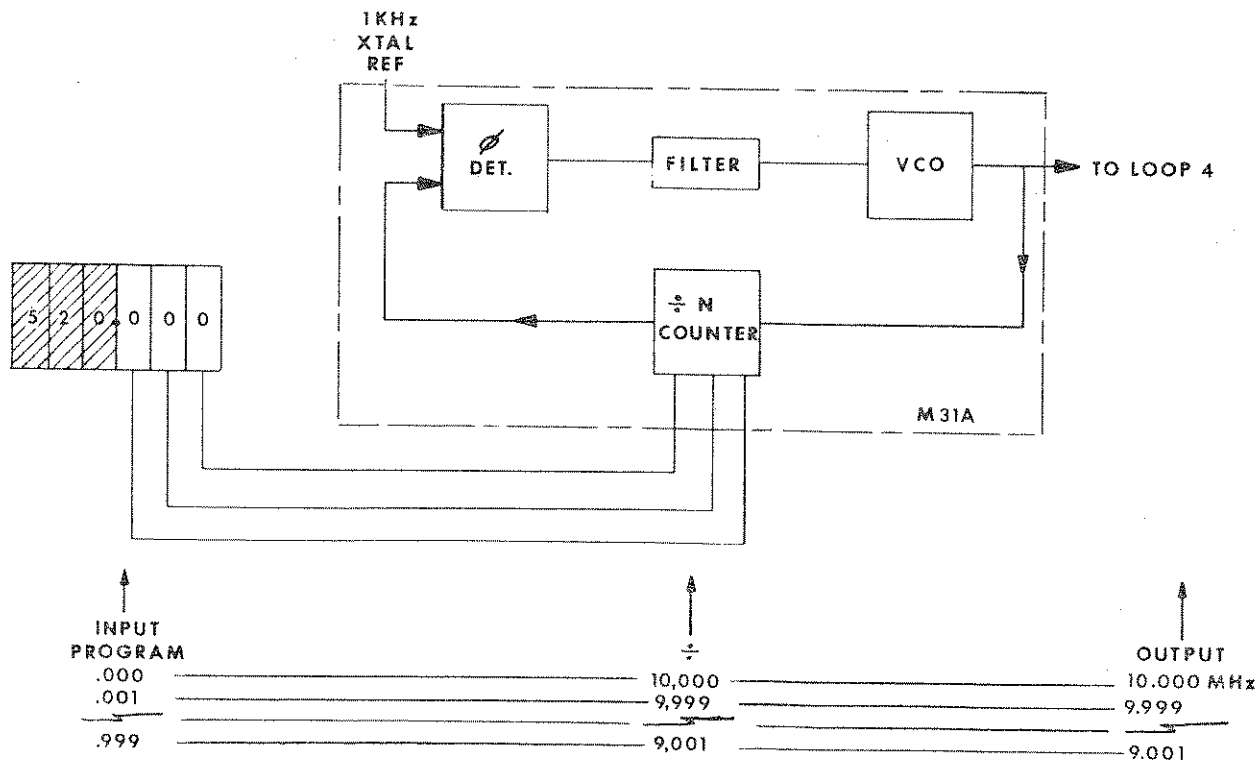
Figure 3-3. PLL 1
