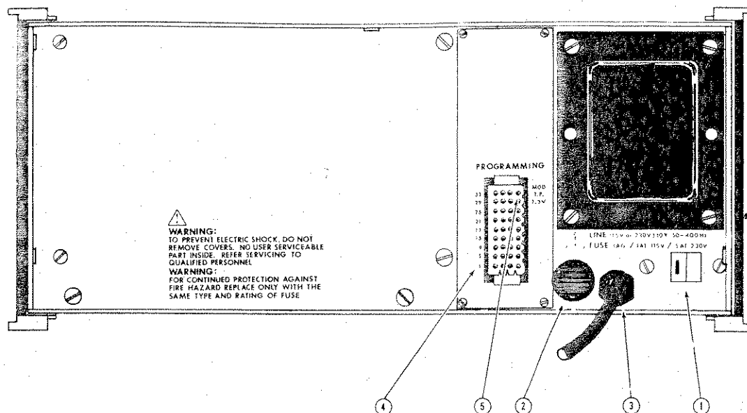
Figure 2-3. Rear Panel
