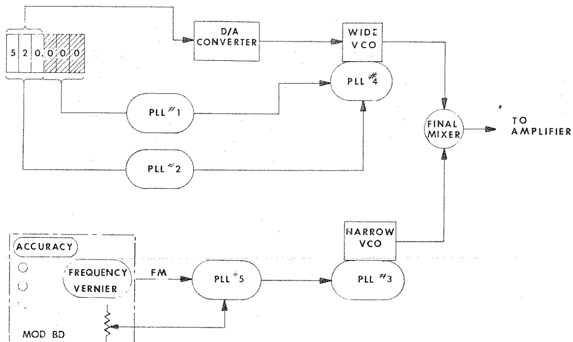
Figure 3-2. PLL Relationships
