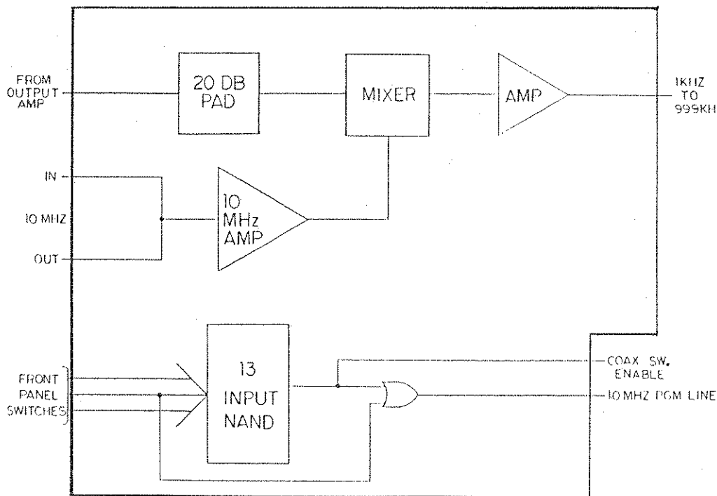
Figure 3-24. M115 Down-Converter
