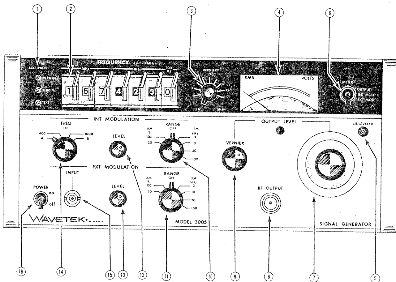
Figure 2-2. Front Panel
