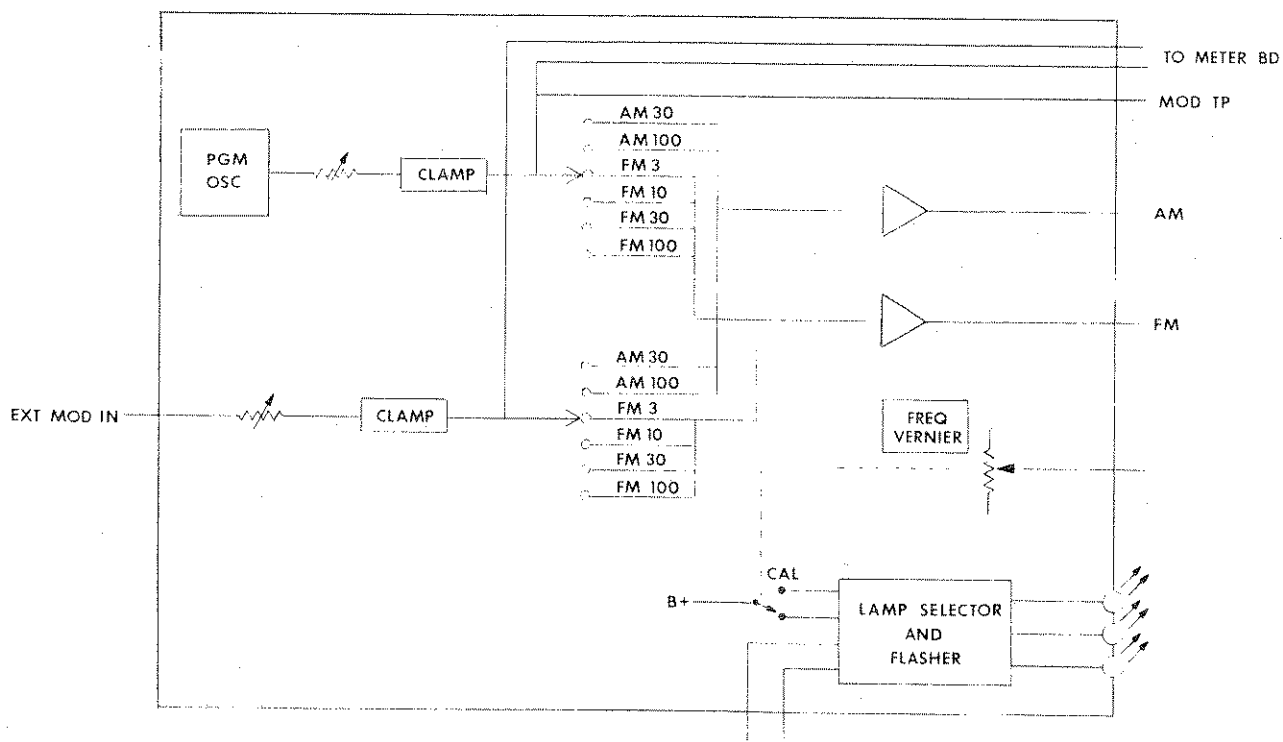
Figure 3-9. Modulation Board
