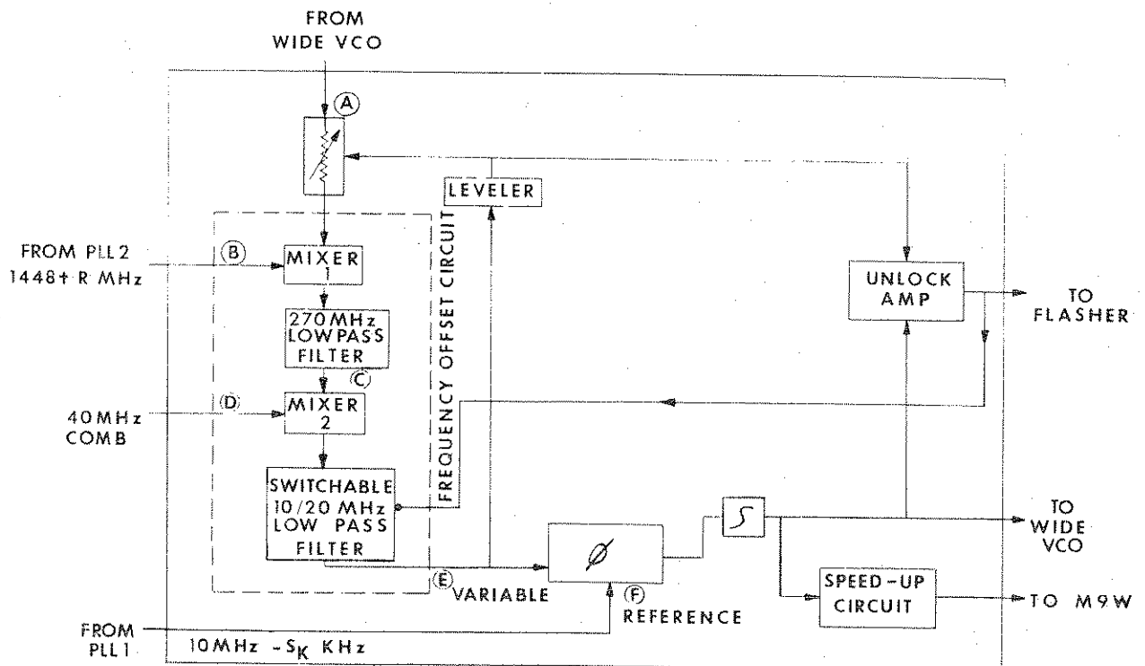
Figure 3-21. M34 Wide Oscillator Lock
