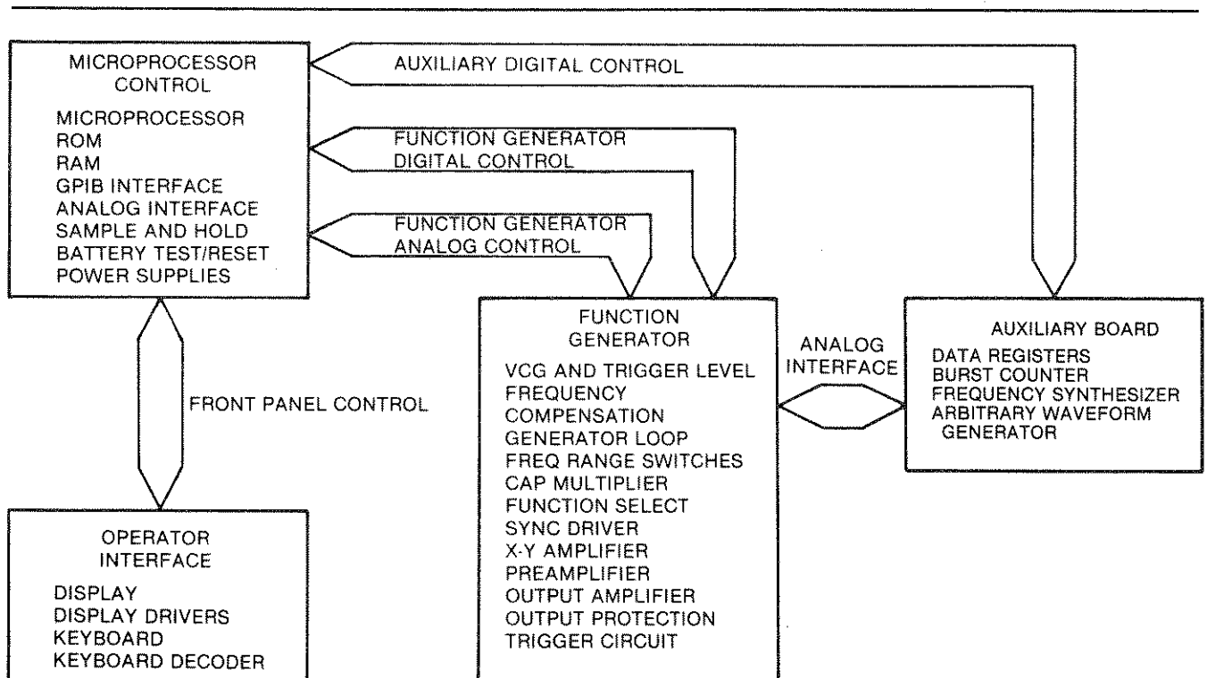
Figure 4-1. Major Blocks
