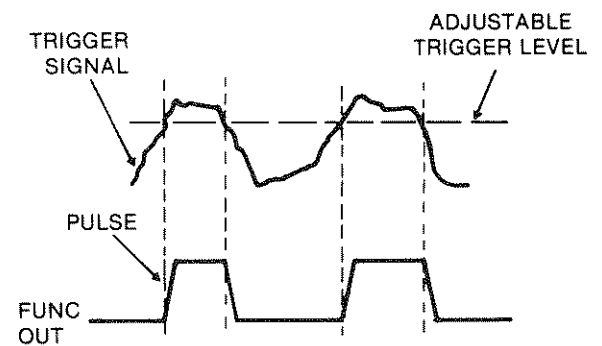
Figure 3-3. External Width
