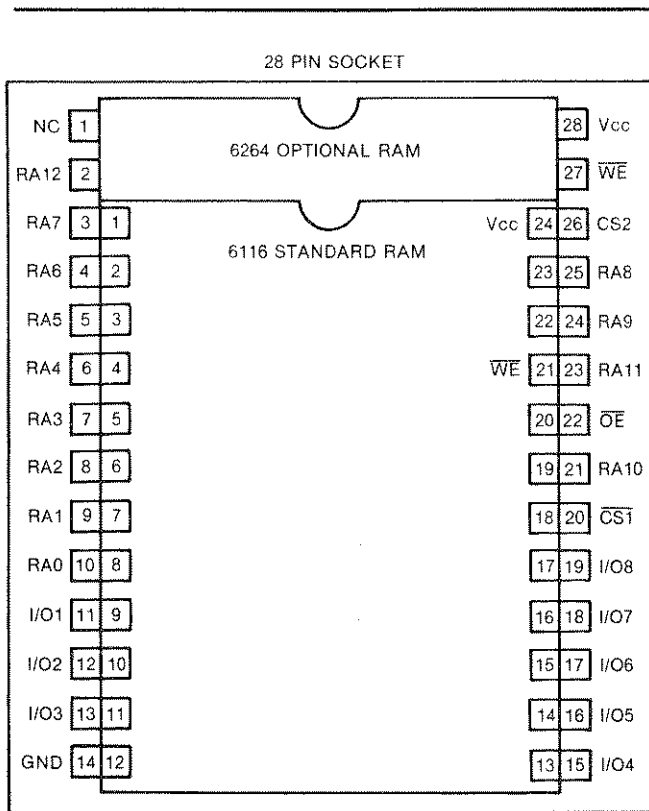
Figure 4-24. ARB RAM Pin Connections
