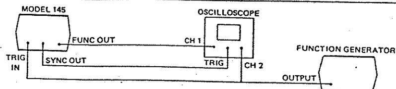
Figure 2-2. Second Setup
