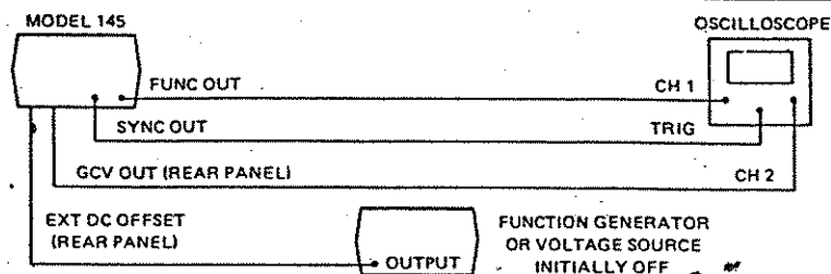
Figure 2-1. Initial Setup
