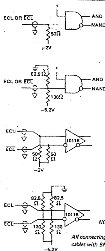
Figure 3-3. ECL Terminations
