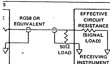
Figure 3-2. Signal Termination
