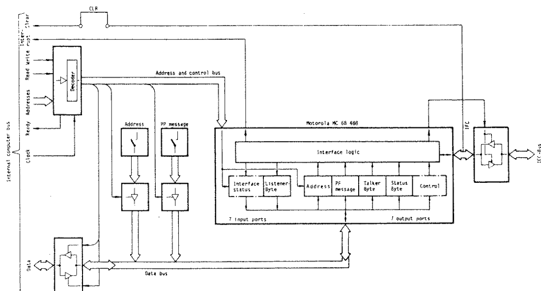
Figure 4-10 Block diagram of the IEC bus interface
