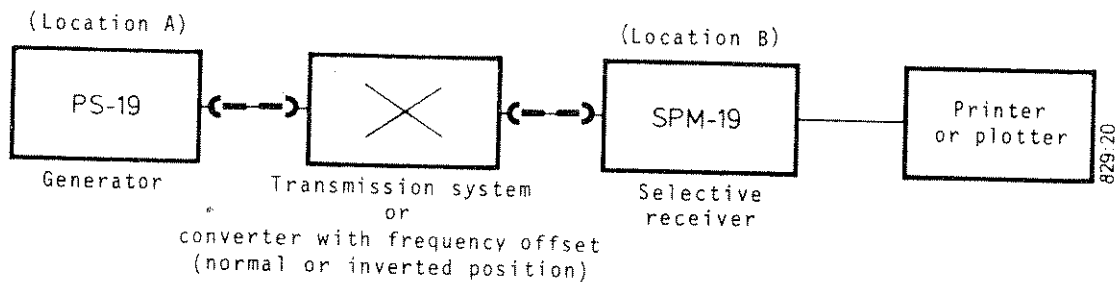
Figure 4-6 Receiver tracking
