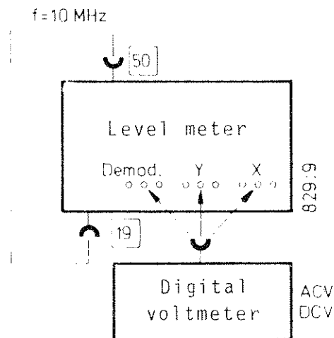
Figure 6-1 Test configuration for the functional test
