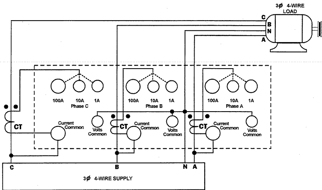
Figure 6-22. Three-Phase Four-Wire CT Source Power Connections
