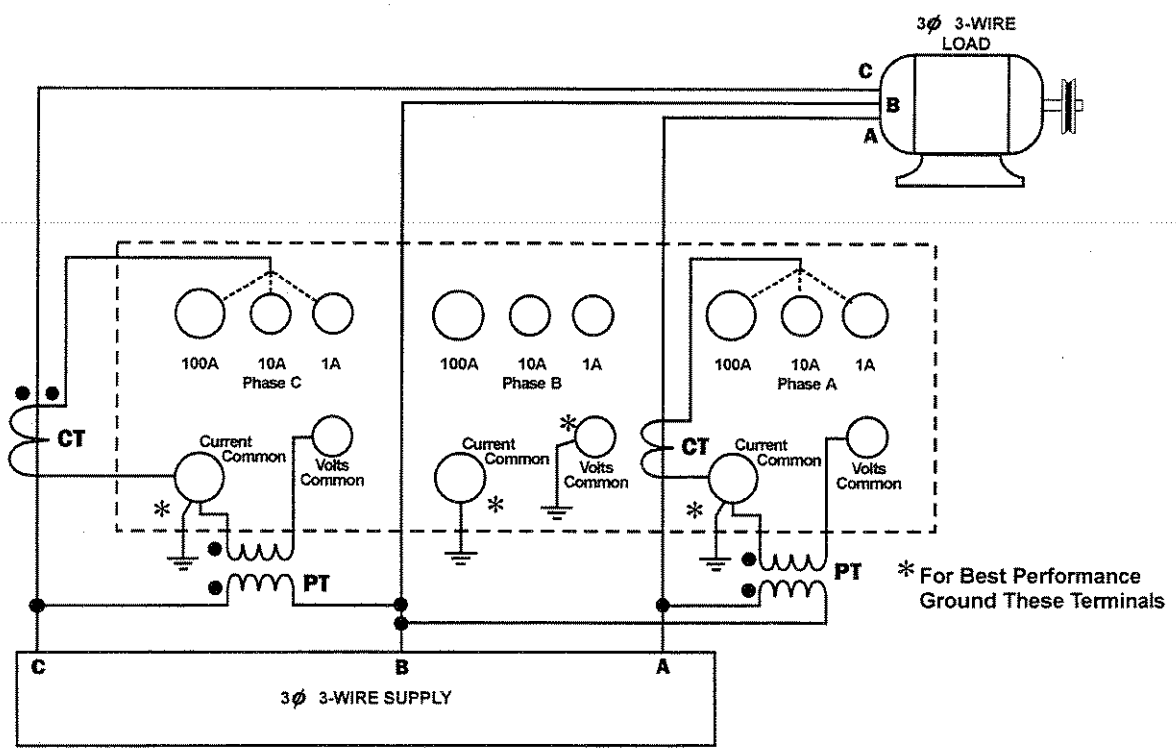
Figure 6-16. Three-Phase Three-Wire CT-PT Source Power Connections
