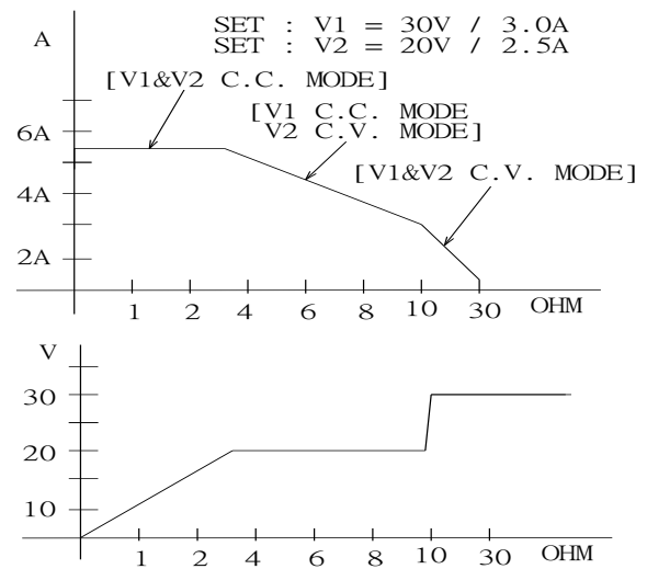
Figure 7 Parallel Voltage/Current Output vs. Load Change
