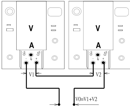
Figure 4 Serial Connection Diagram
