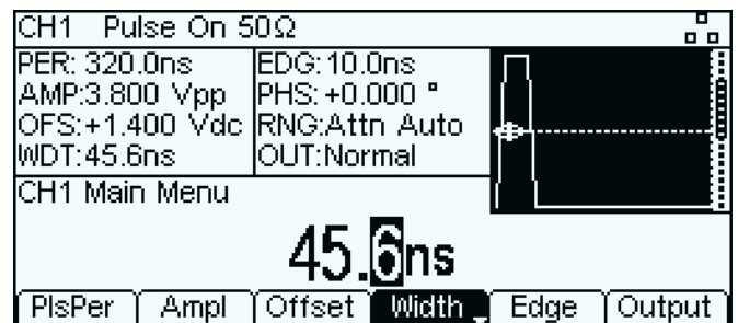
Pulse width and edge speeds can be set to a resolution of 0.1ns (100ps)
