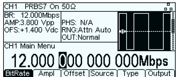
PRBS patterns of 8 sequence lengths up to 50Mbps
