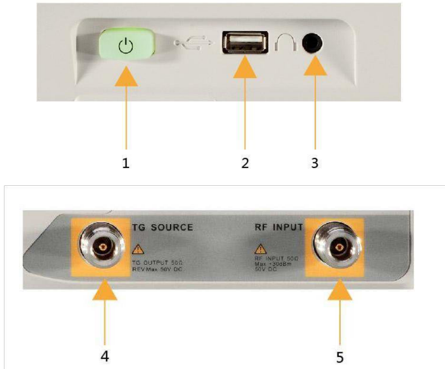
Figure 1-9 Front Panel Connectors
