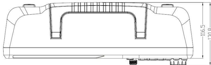
Figure 1-2 Top View
