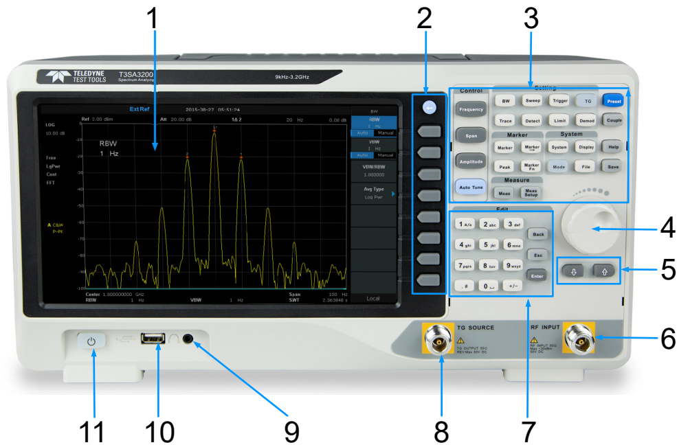
Figure 1-6 The Front Panel
