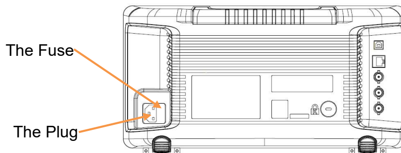
Figure 1-5 Power Cord Connection
