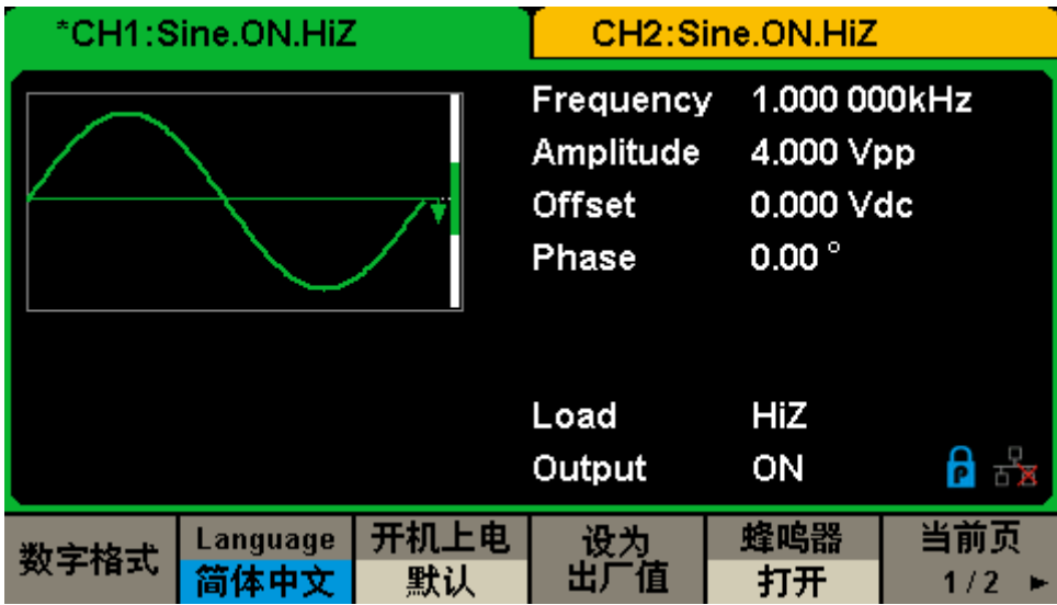
Figure 2-49 Chinese Interface
