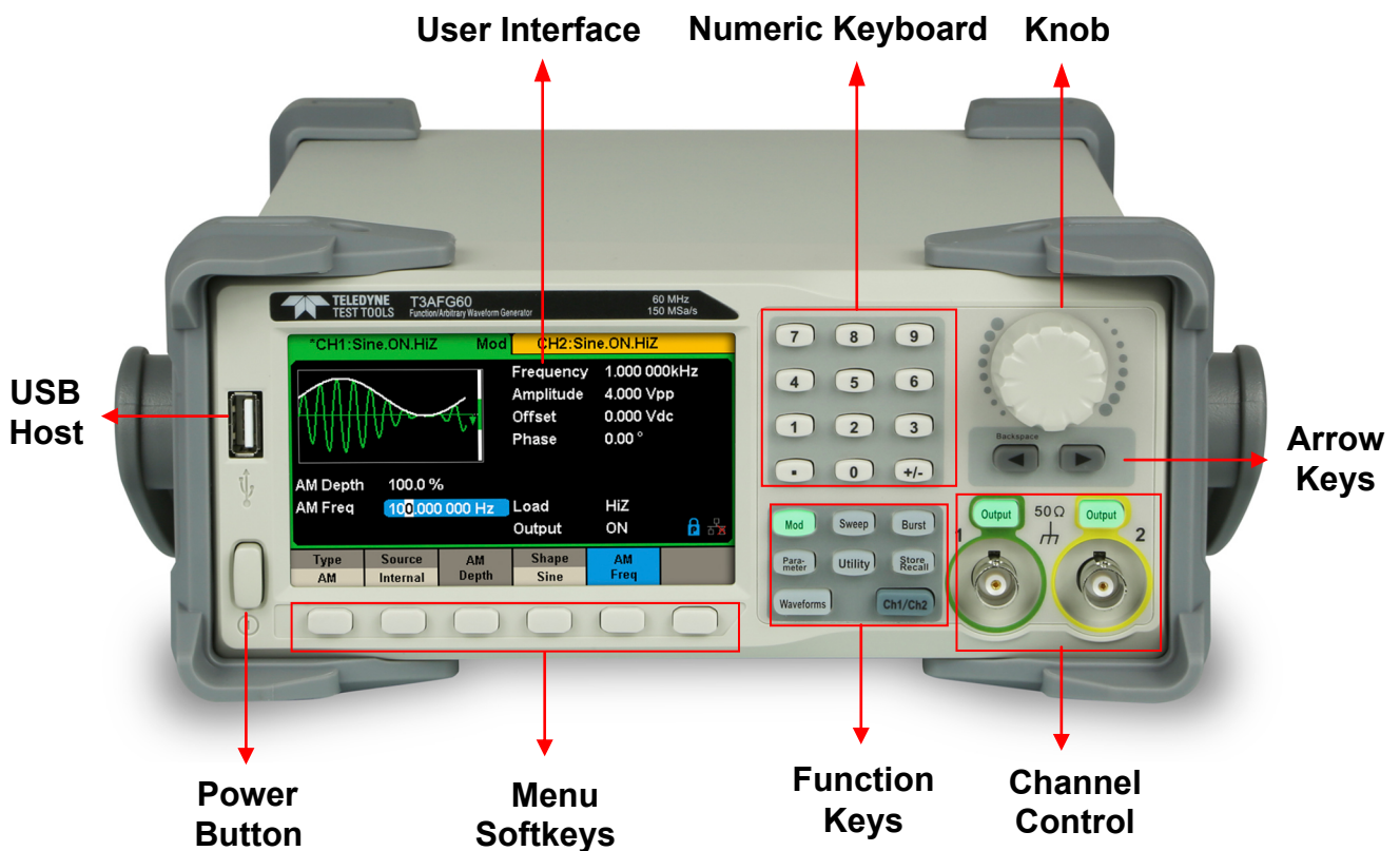
Figure 1-2 Front Panel
