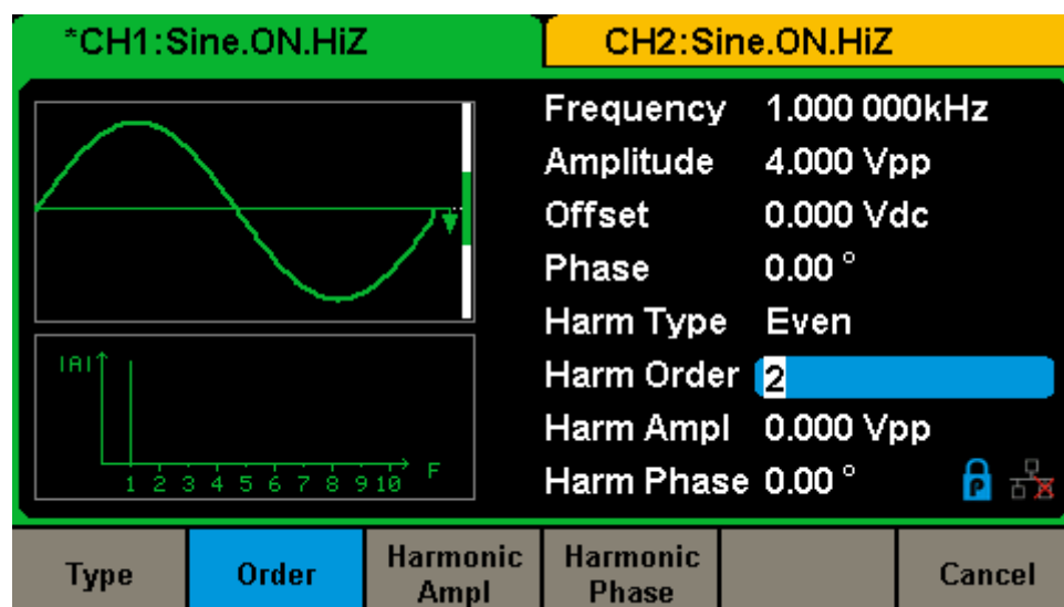
Figure 2-20 Harmonic Interface
