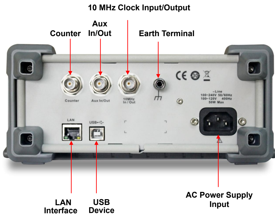
Figure 1-3 Rear Panel
