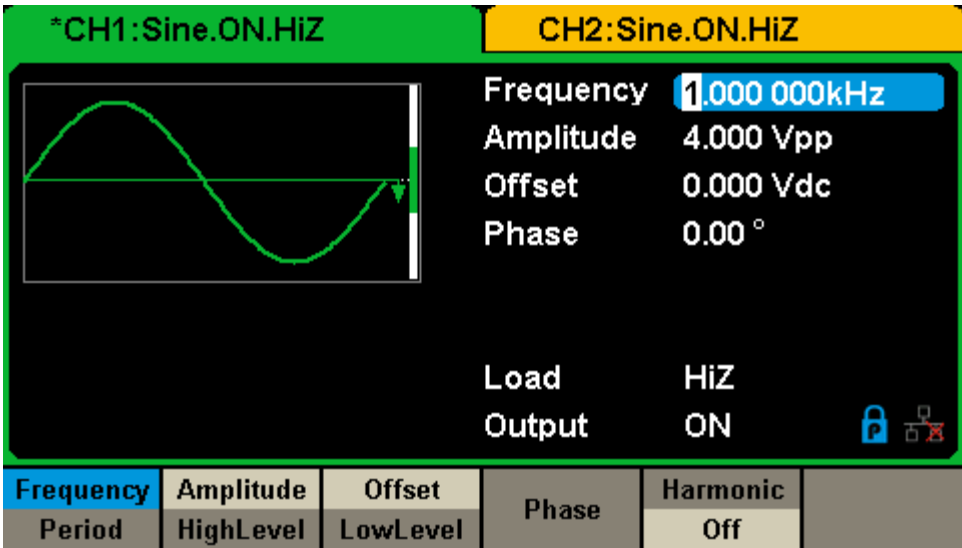
Figure 2-71 Phase-locked Mode
