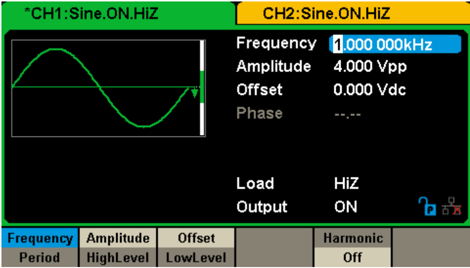
Figure 2-72 Independent Mode
