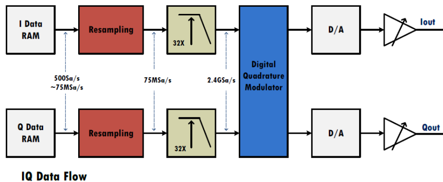
Figure 2-29 IQ modulation
