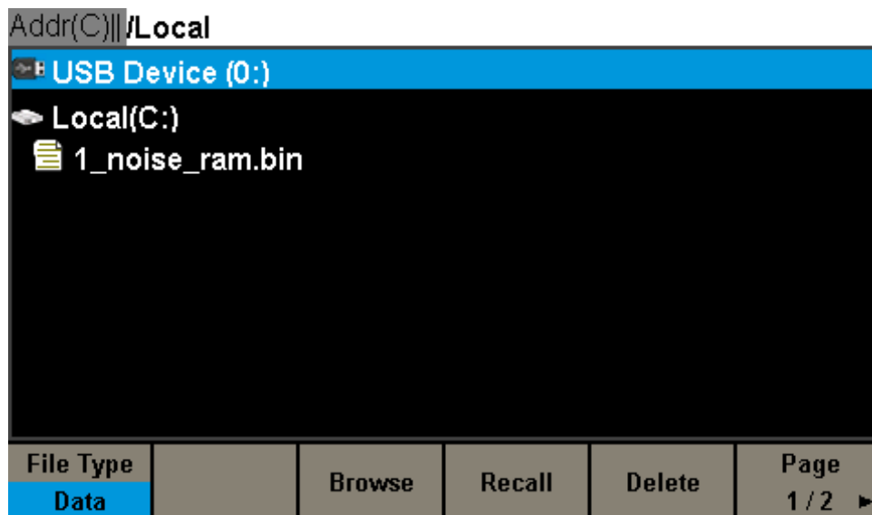
Figure 2-44 Storage System
