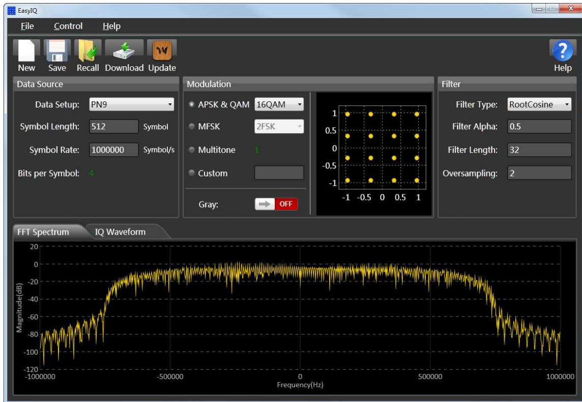
Figure 2-36 EasyIQ Interface
