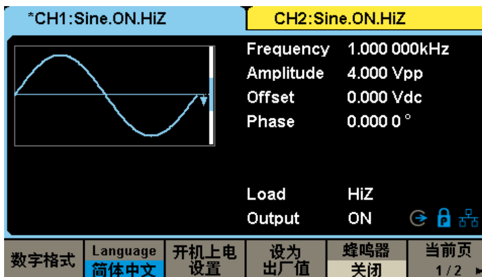
Figure 2-52 Chinese Interface
