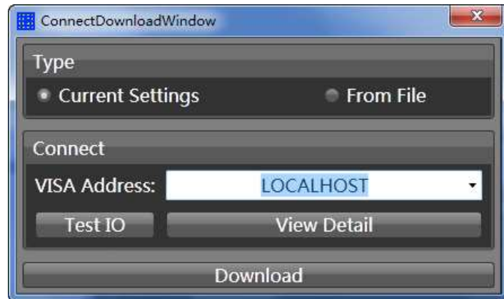
Figure 2-45 Download Interface
