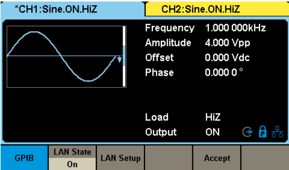
Figure 2-72 Interface Settings
