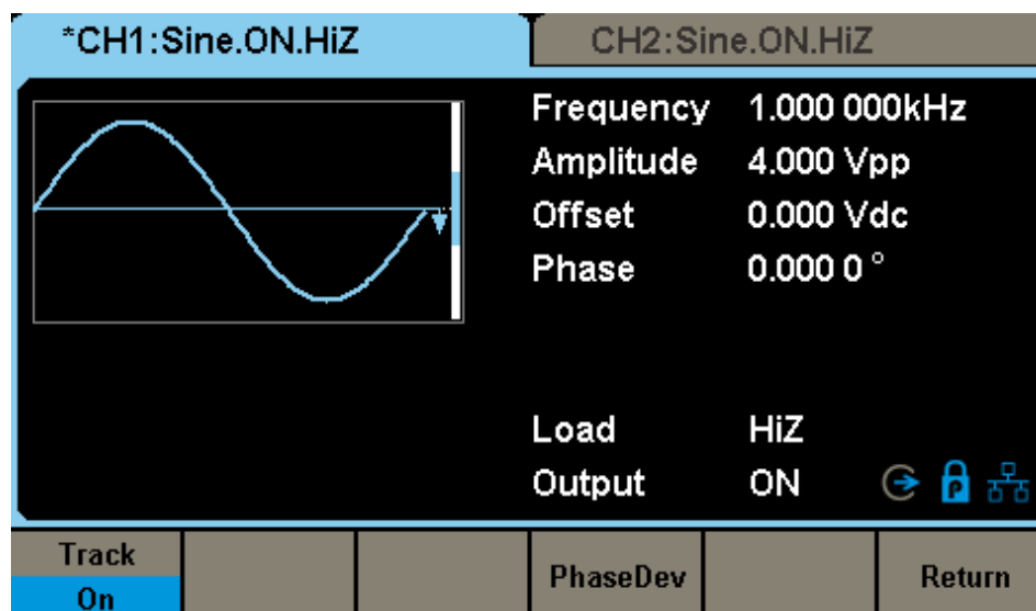
Figure 2-70 Track Interface
