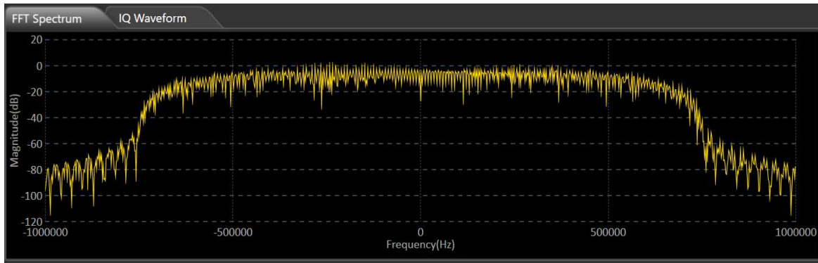
Figure 2-43 Waveform Spectrum
