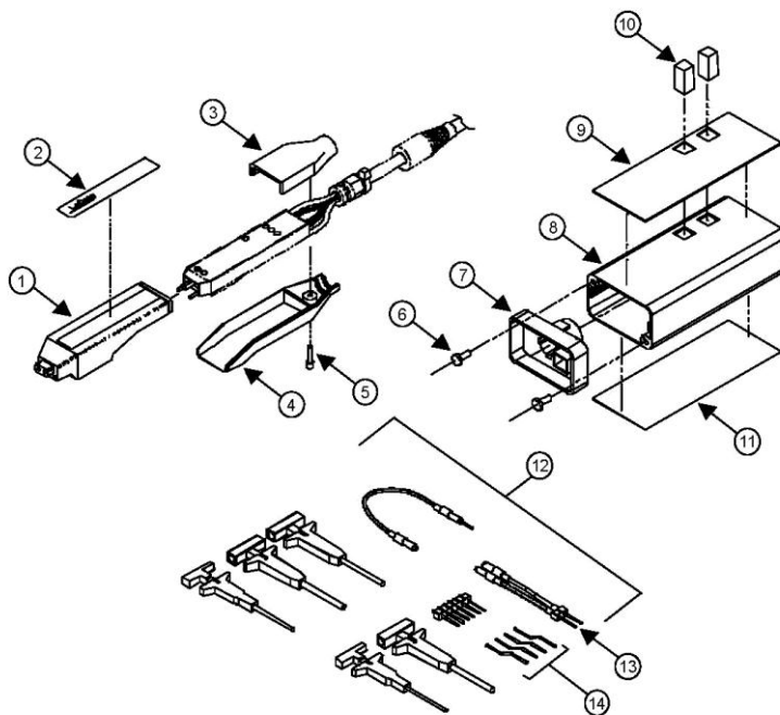
Figure 6, Replaceable Parts
