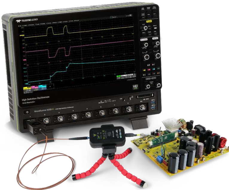
Probe elevated above DUT
