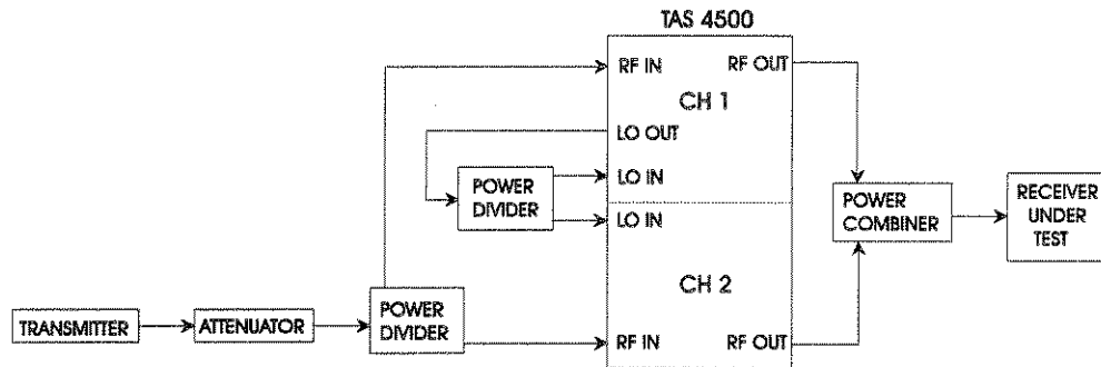
Figure 1-5. Single Channel 12 Path Configuration
