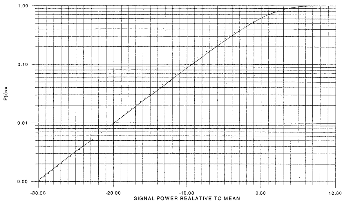
Figure 3-9. Measured vs. Theoretical CPDF
