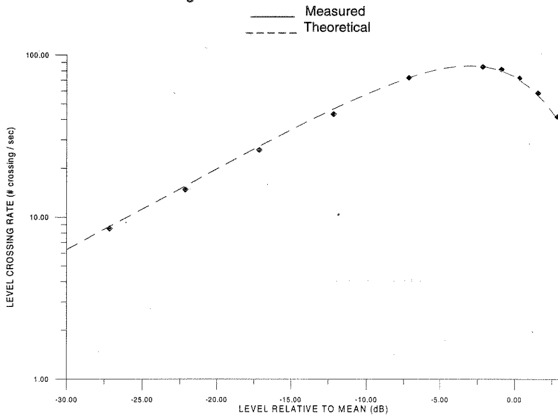
Figure 3-10. Measured vs. Theoretical LCR
