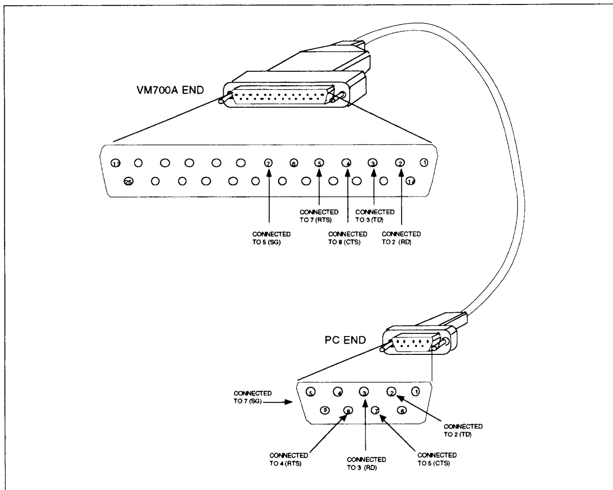
Figure 2-2. Pin Configuration for VM700A 25-Pin to PC 9-Pin Cable.
