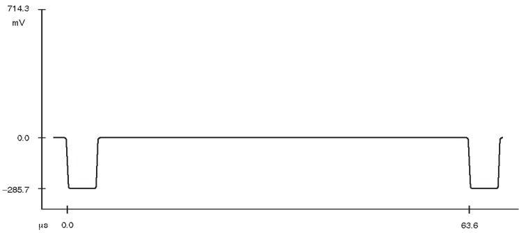
Figure 11: 0 IRE, No Burst
