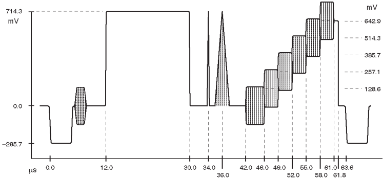
Figure 2: NTC7 Composite
