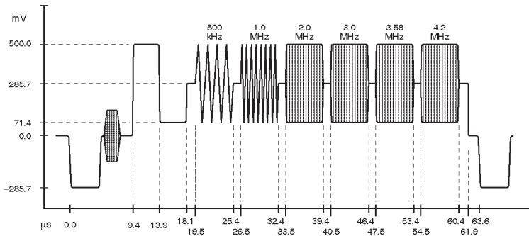
Figure 1: Multiburst
