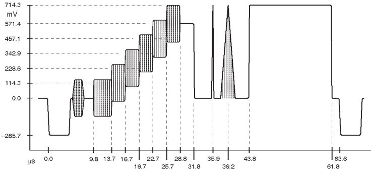
Figure 4: FCC Composite
