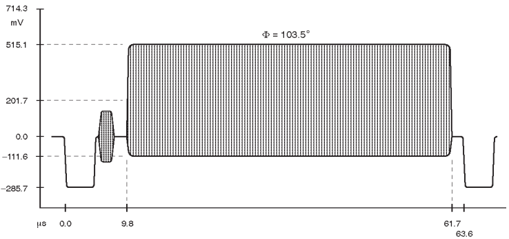
Figure 8: Red Field
