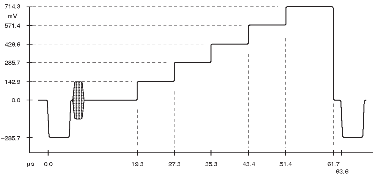
Figure 7: 5-Step Staircase (Gray Scale)
