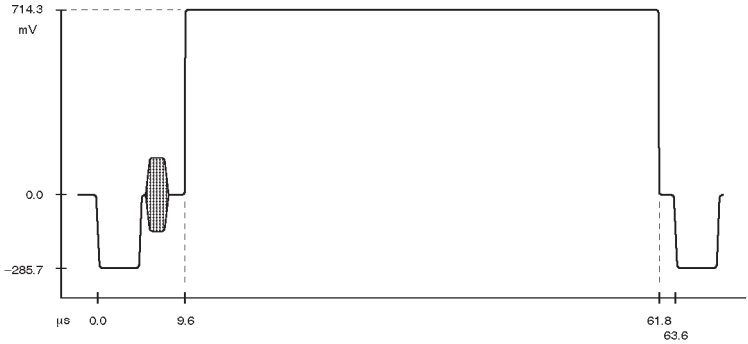
Figure 9: Field Square Wave
