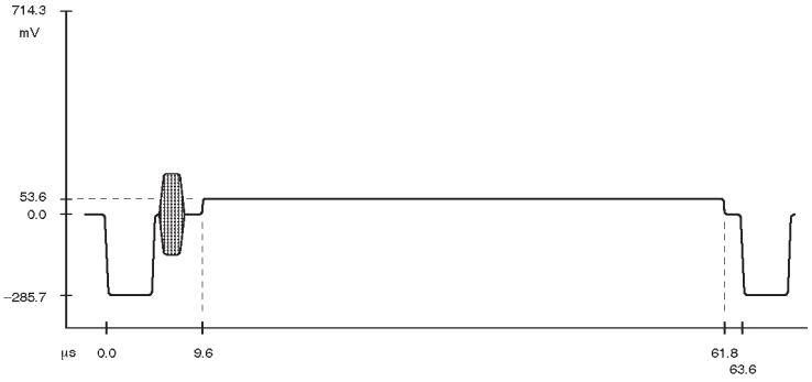
Figure 12: Black Burst
