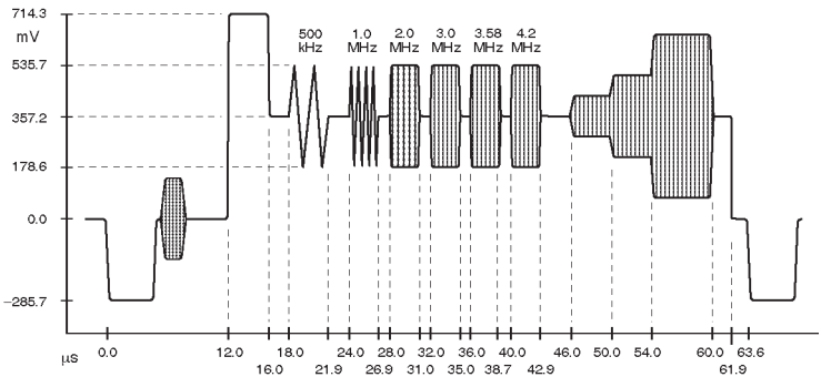
Figure 3: NTC7 Combination
