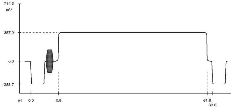
Figure 10: 50 IRE Flat Field
