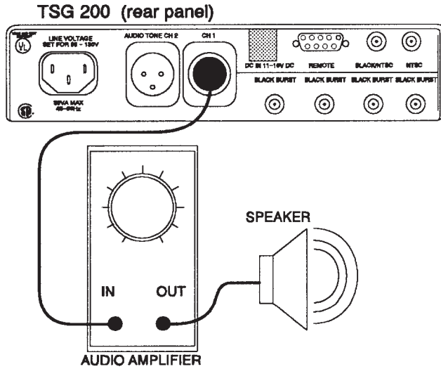
Fig. 4-6. Audio ID click frequency adjustment setup.
