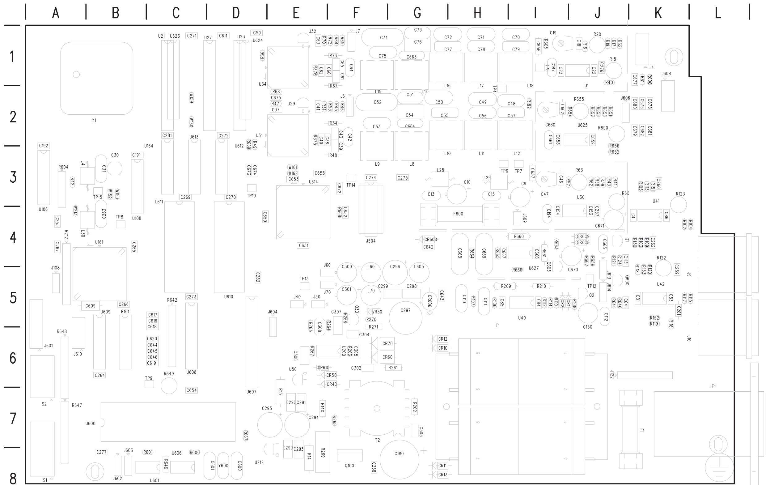
A2 MAIN BOARD 070-1927-03 (Std) 070-2507-03 (Opt 1J)
