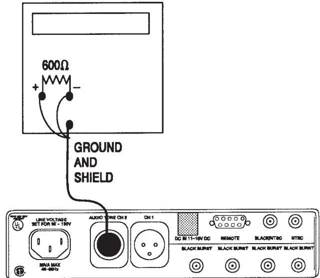
Fig. 4-3. Setup to measure the total harmonic distortion.
