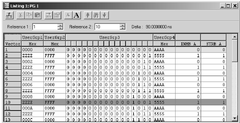
Figure 7: Listing window
