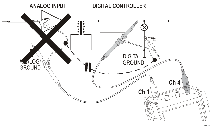
Figure 2-7: Wrong connection of reference leads
