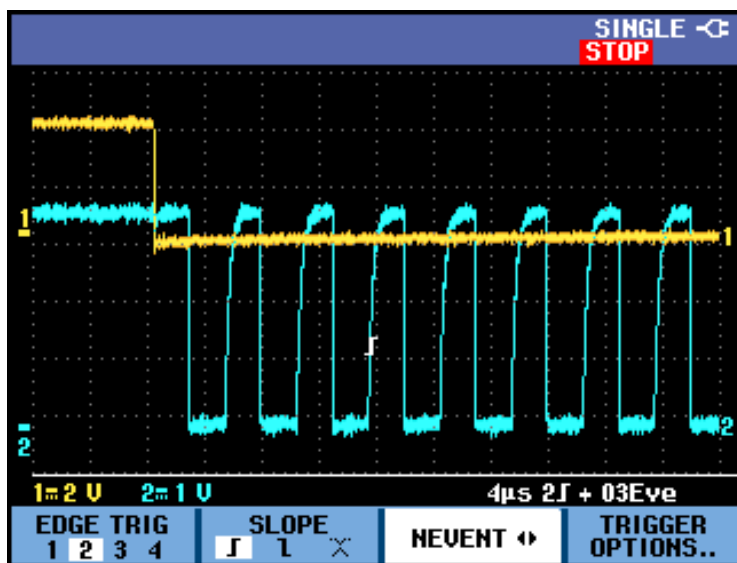
Figure 3-11: N-Event triggering
