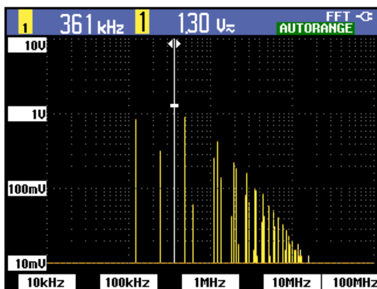
Figure 2-18: FFT measurement
