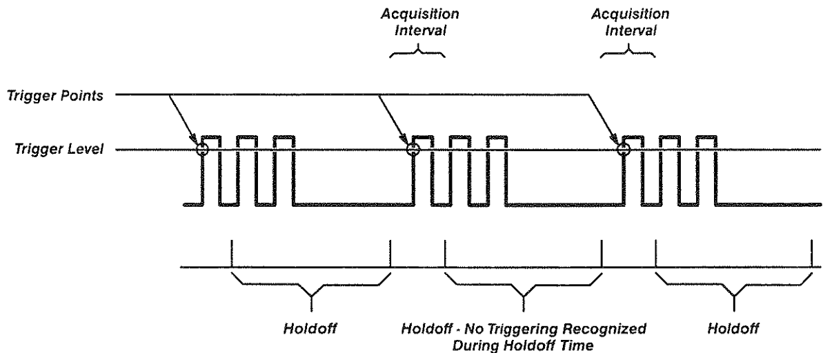
Figure 2-6: Trigger Holdoff Time Ensures Valid Triggering
