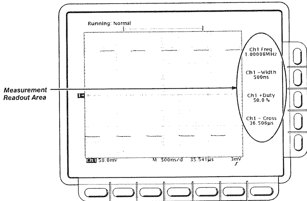
Figure 3-32: Measurement Readouts
