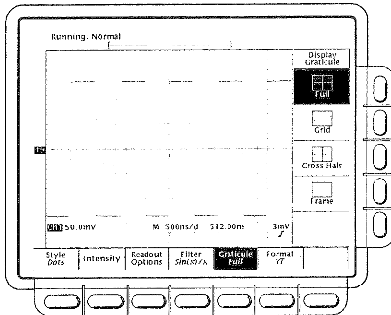
Figure 3-13: Display Menu—Graticule
