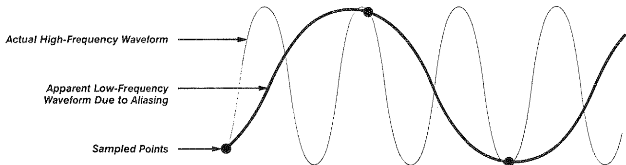
Figure 2-12: Aliasing
