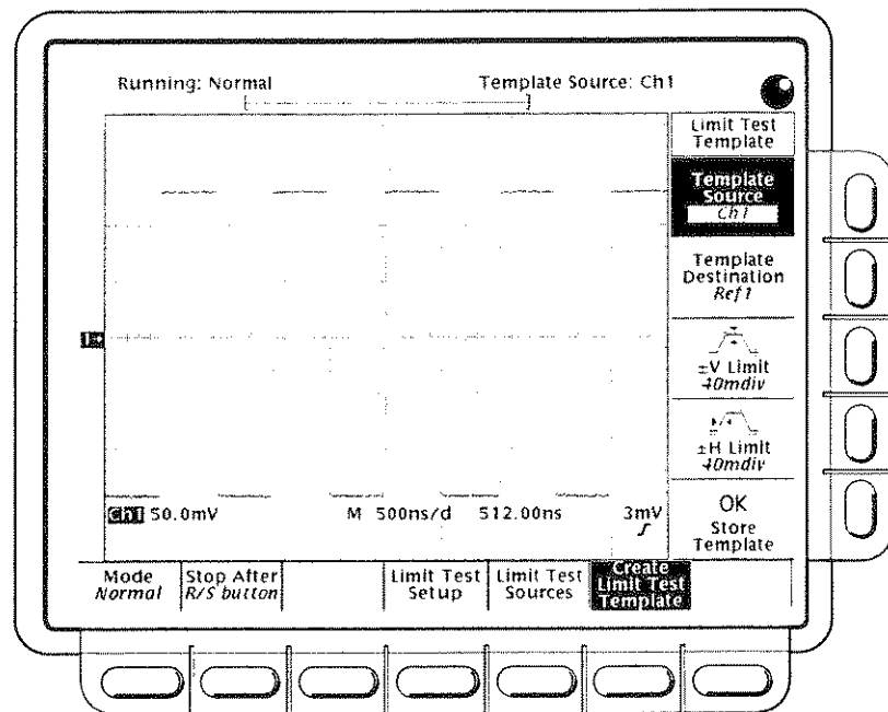
Figure 3-29: Acquire Menu—Create Limit Test Template
