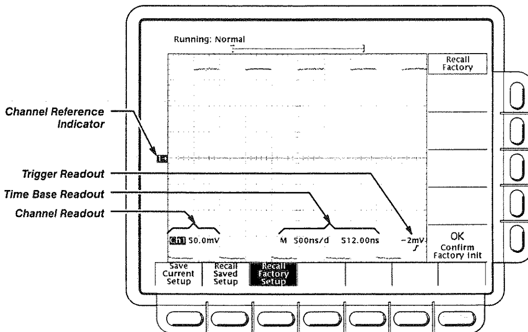
Figure 1-9: Display Elements
