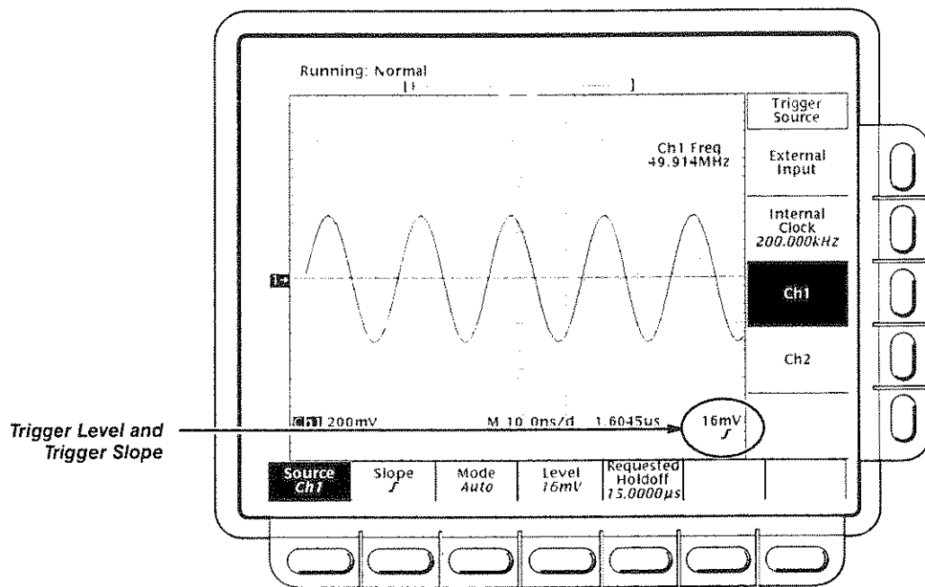
Figure 3-60: Example Trigger Readouts
