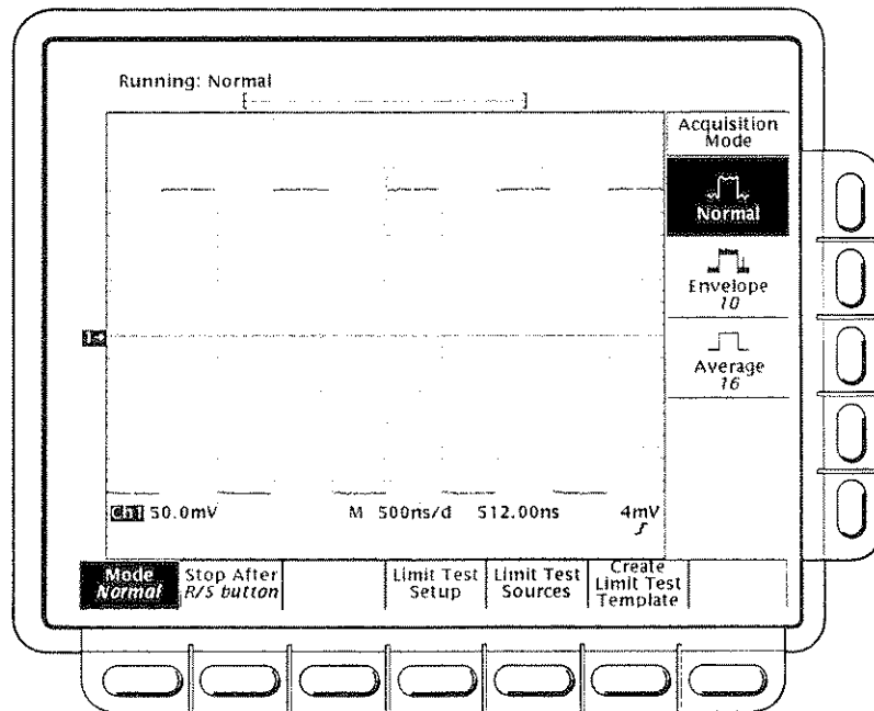
Figure 3-2: Acquire Menu
