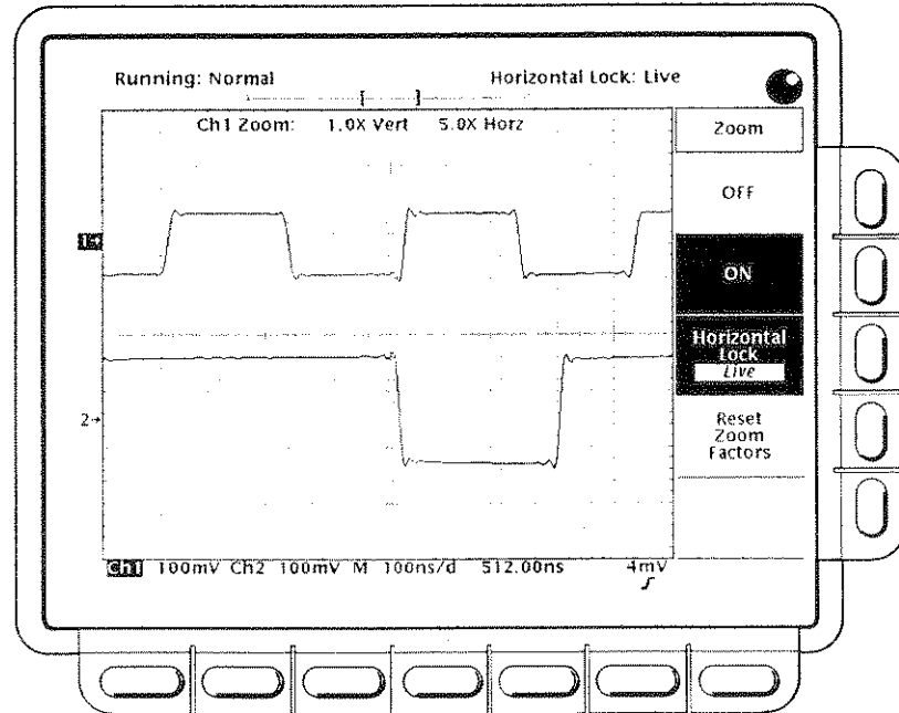
Figure 3-74: Zoom Mode with Horizontal Lock Set to Live
