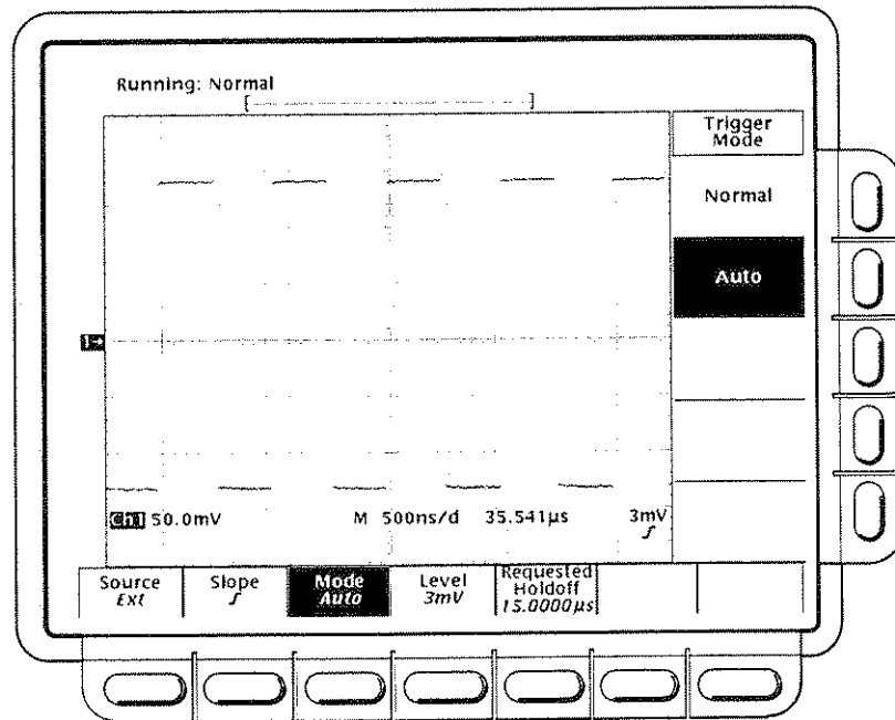
Figure 3-64: Trigger Menu—Mode
