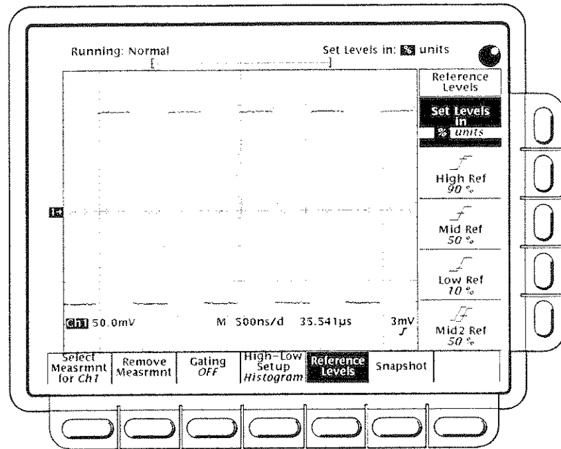
Figure 3-36: Measure Menu—Reference Levels
