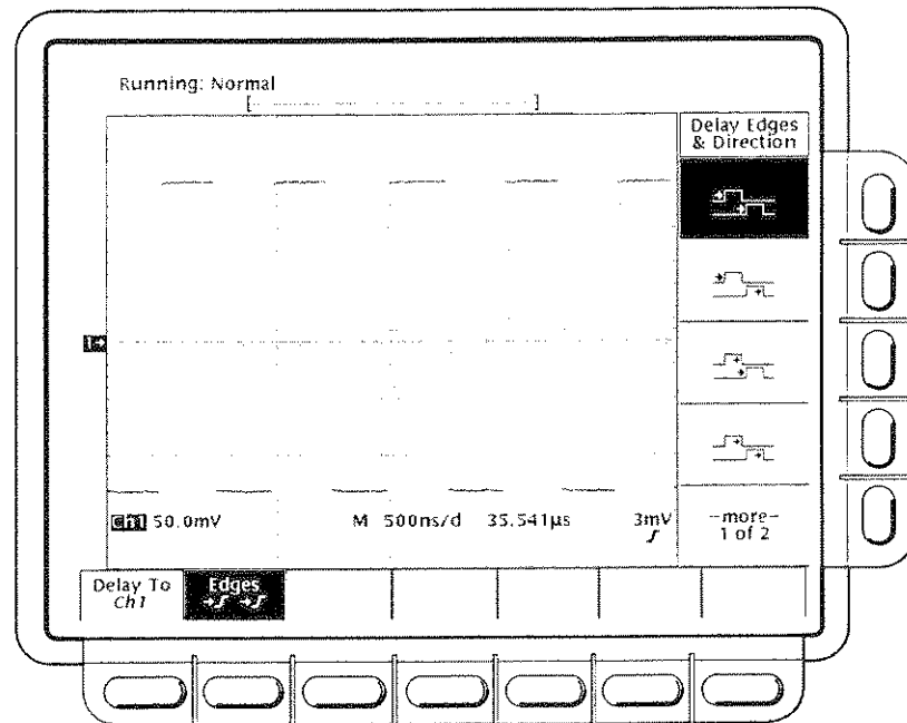
Figure 3-38: Measure Delay Menu—Edges
