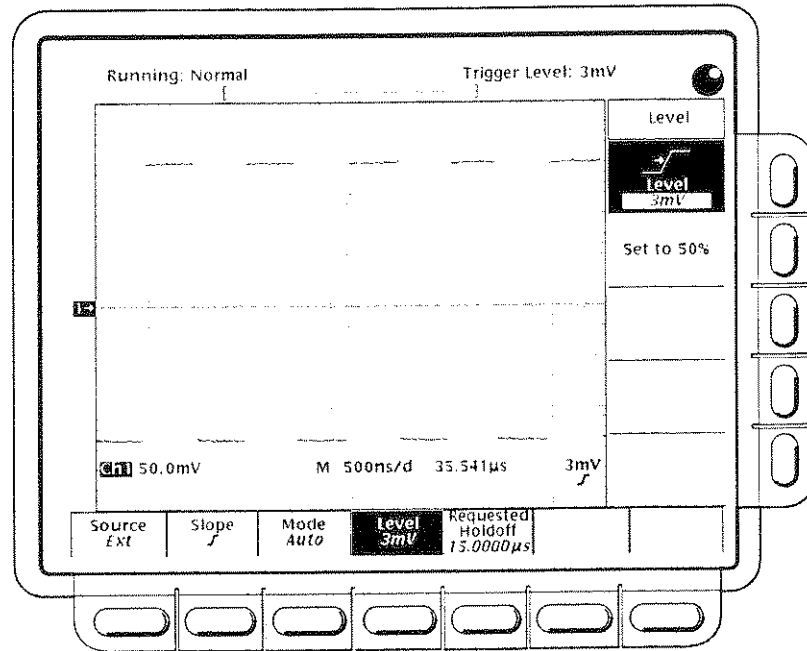
Figure 3-65: Trigger Menu—Level
