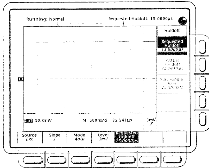
Figure 3-66: Trigger Menu—Holdoff
