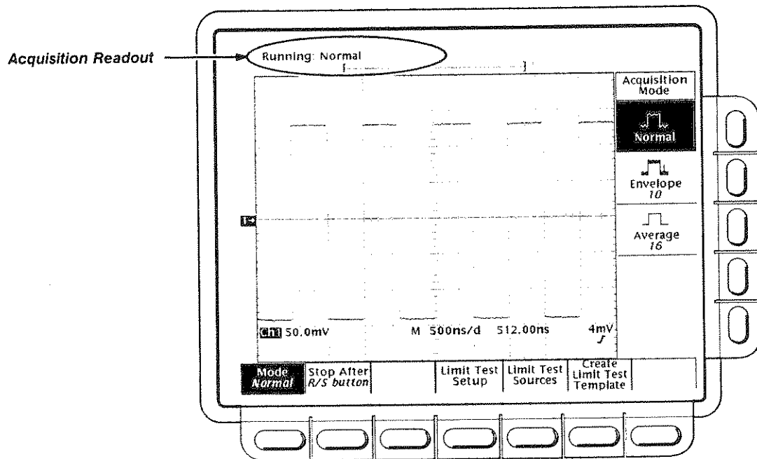
Figure 3-1: Acquisition Readout
