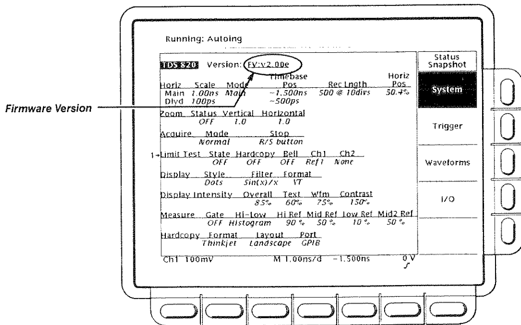
Figure 3-57: Status Menu—System
