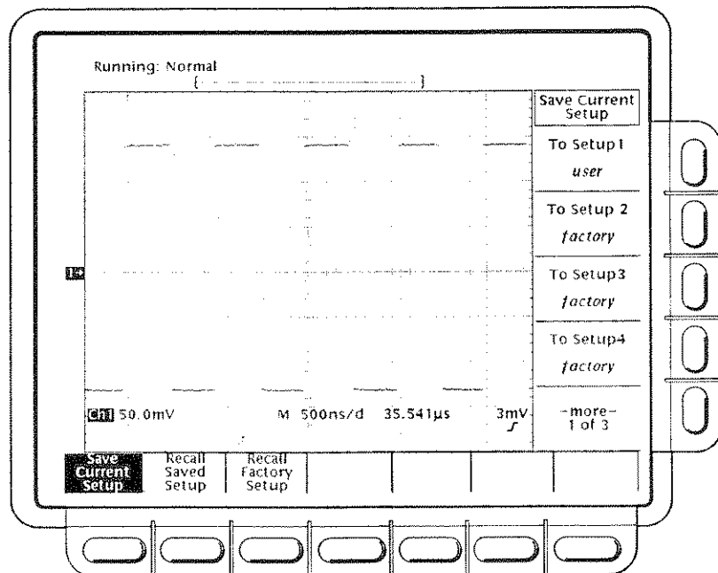
Figure 3-51: Save/Recall Setup Menu
