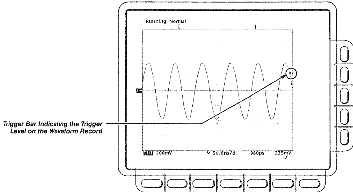
Figure 3-62: Trigger Level Bar Readout
