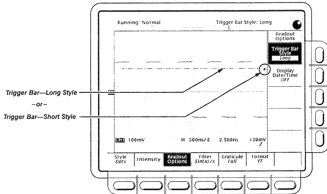
Figure 3-12: Level Indicators
