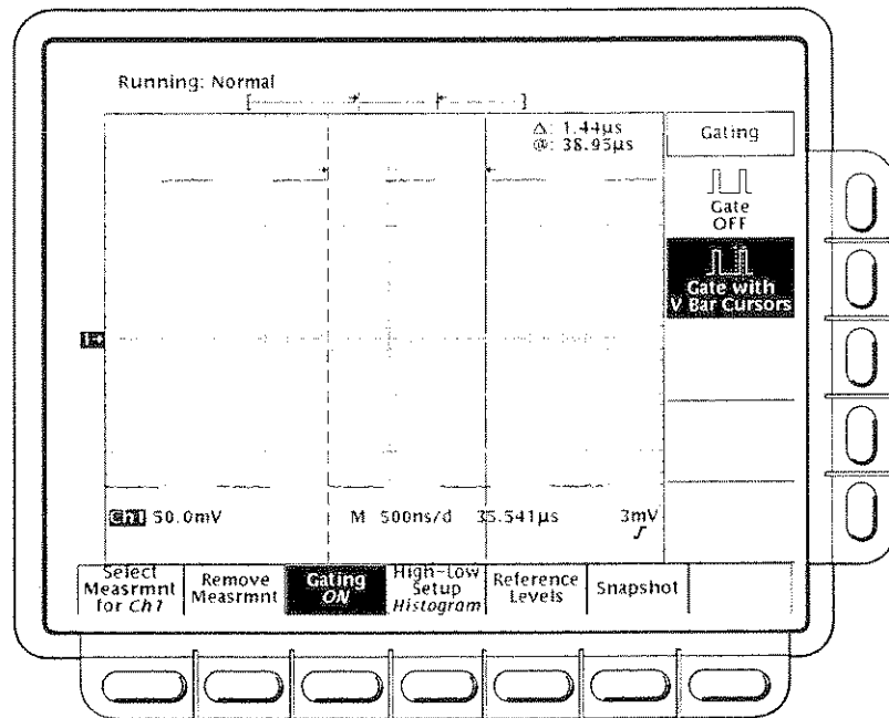
Figure 3-34: Measure Menu—Gating
