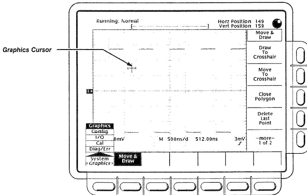
Figure 3-15: Graphics Menu
