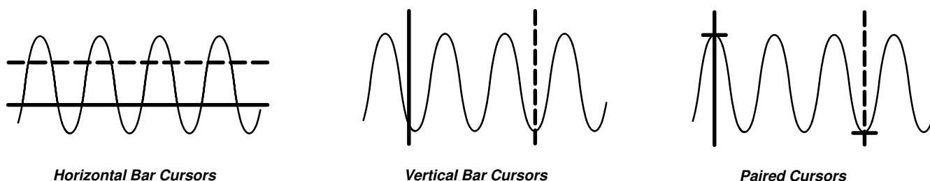
Figure 3-4: Cursor Types
