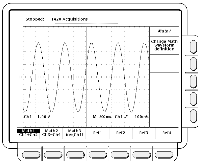
Figure 3-63: More Menu
