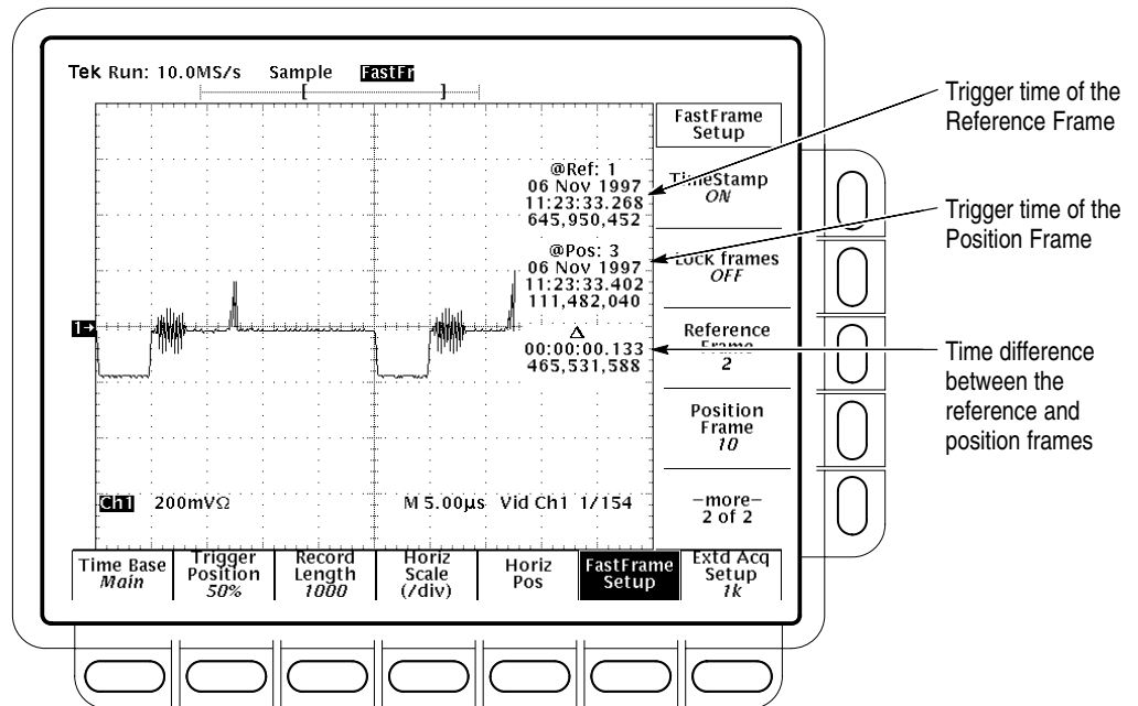
Figure 3–35: FastFrame TimeStamp
