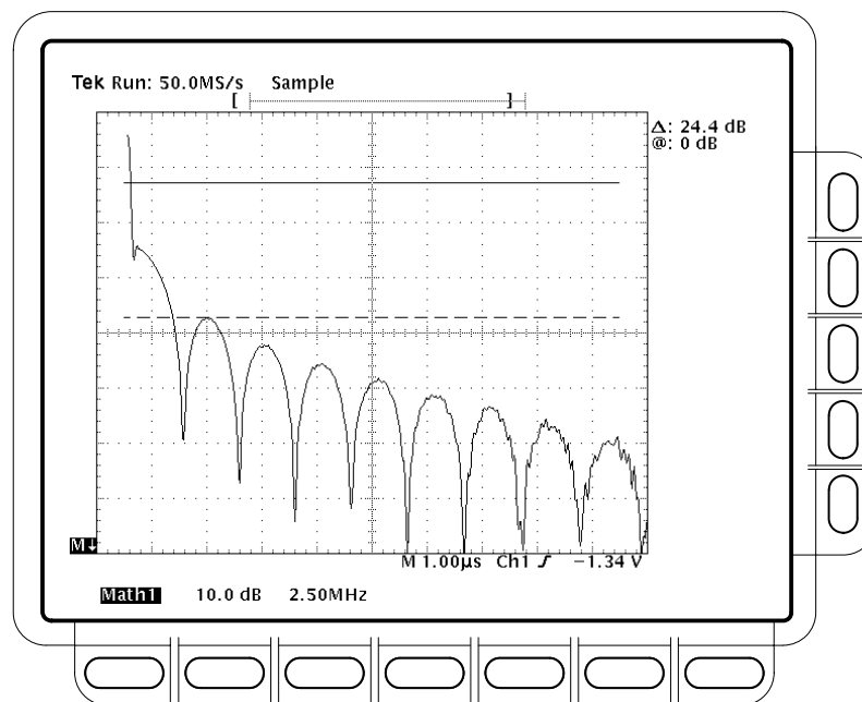
Figure 3–99: Cursor Measurement of an FFT Waveform
