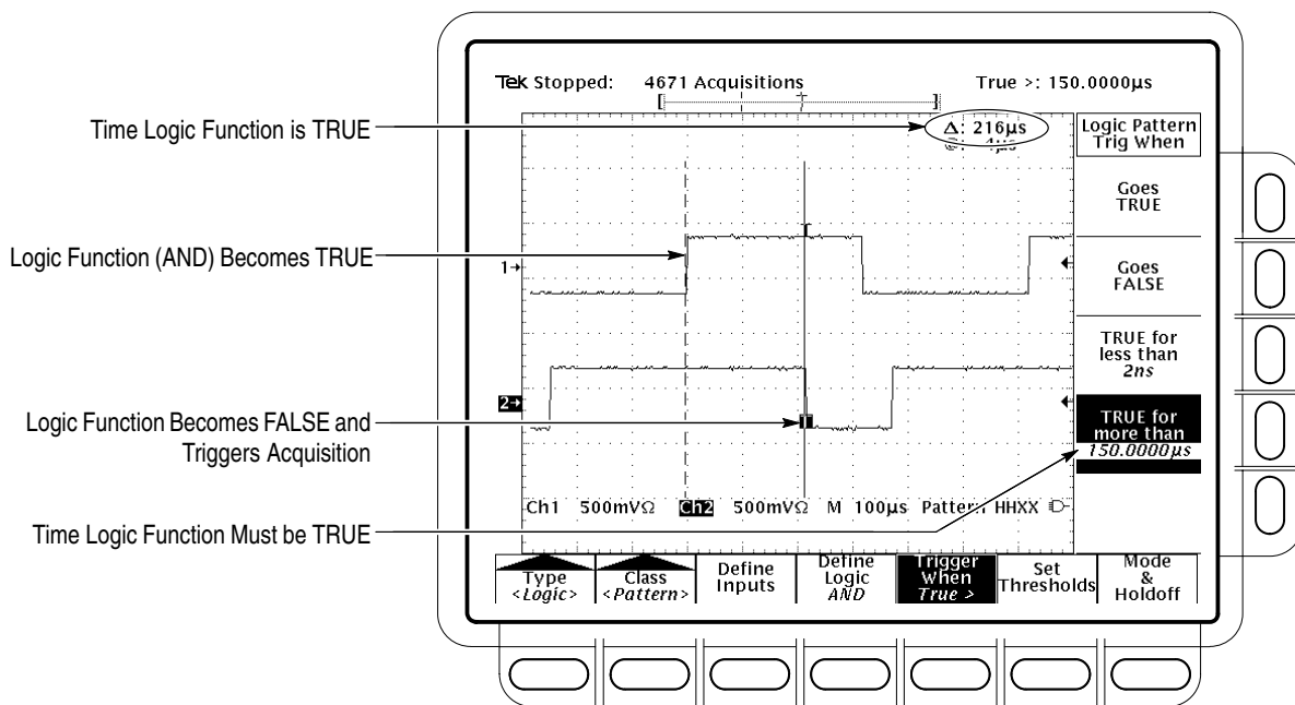
Figure 3–47: Logic Trigger Menu — Time Qualified TRUE
