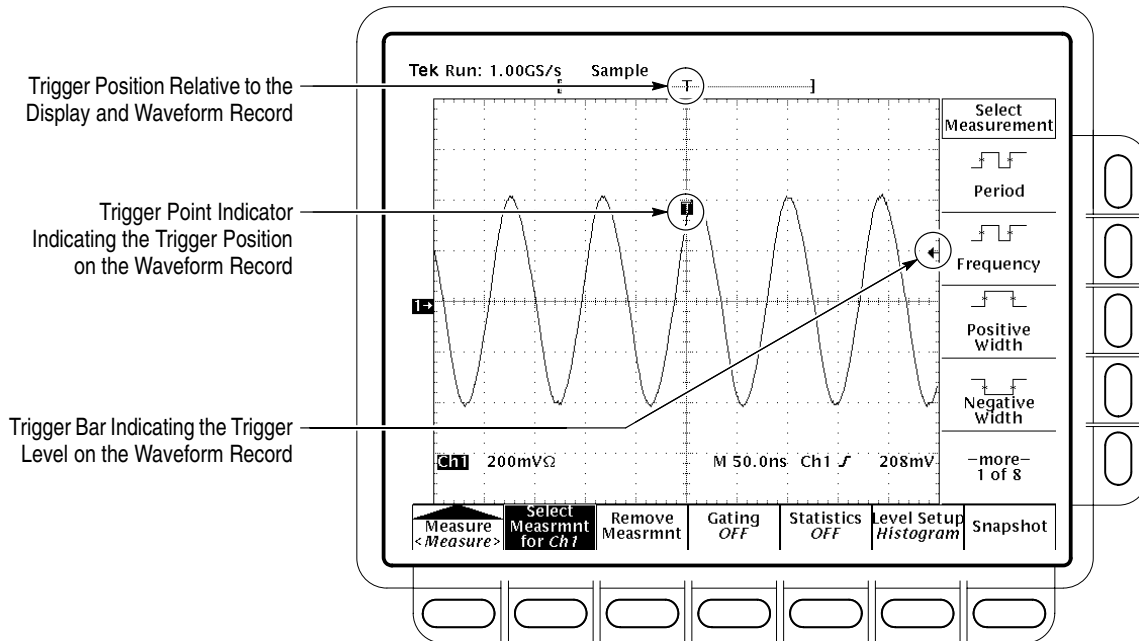
Figure 3-41: Record View, Trigger Position, and Trigger Level Bar Readouts
