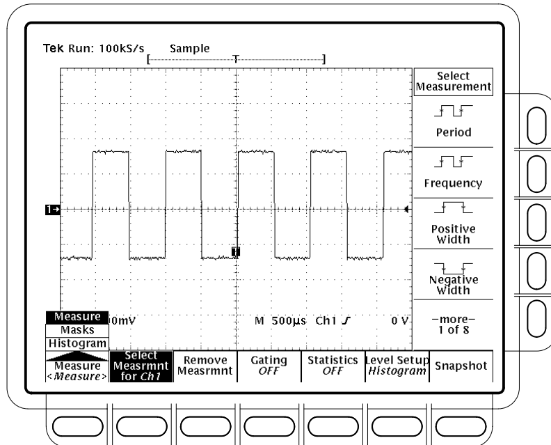
Figure 3–60: Measure Menu
