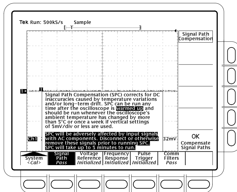
Figure 3–72: Performing a Signal Path Compensation
