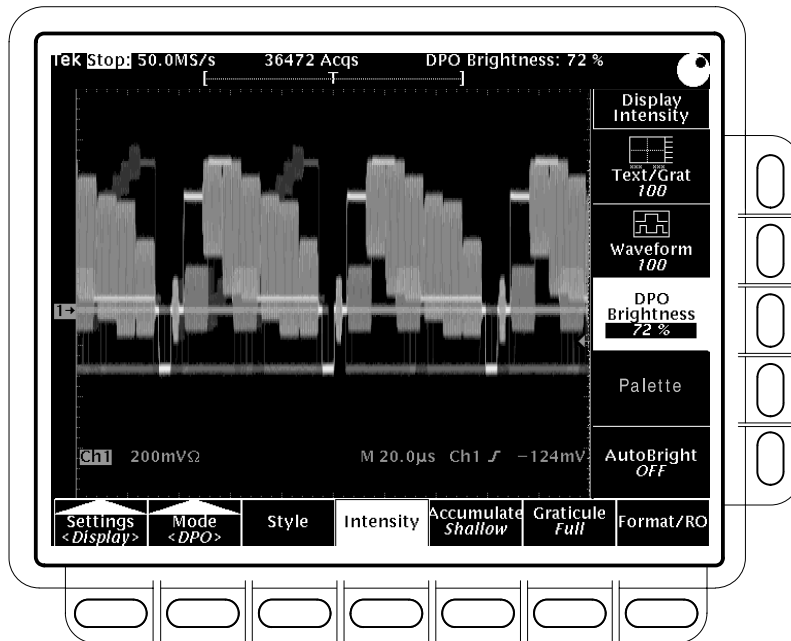
Figure 3–29: DPO Display
