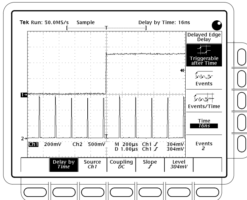
Figure 3–57: Delayed Trigger Menu
