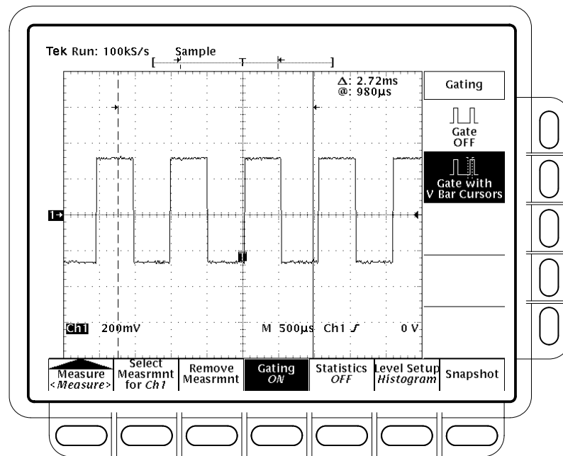
Figure 3–61: Measure Menu — Gating
