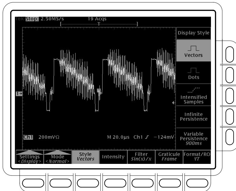
Figure 3–30: Normal DSO Display
