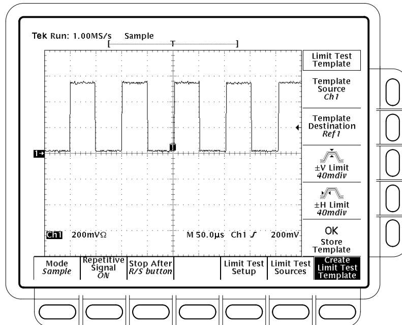
Figure 3-93: Acquire Menu — Create Limit Test Template
