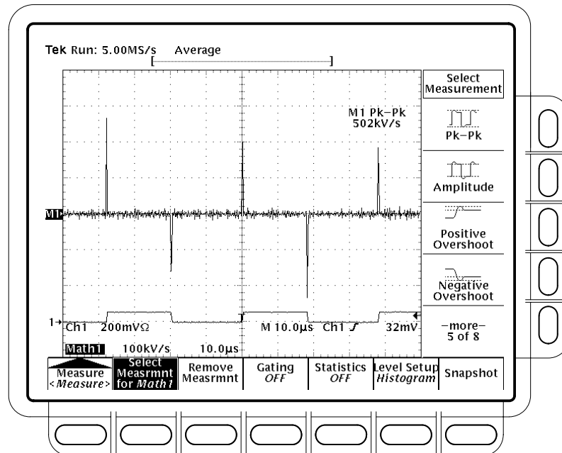
Figure 3–106: Peak-Peak Amplitude Measurement of a Derivative Waveform
