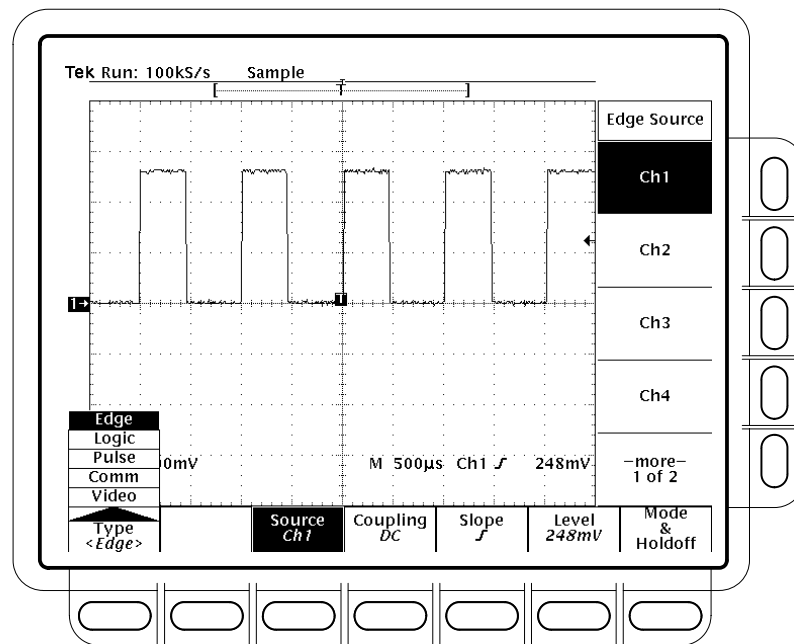
Figure 3-43: Main Trigger Menu — Edge Type
