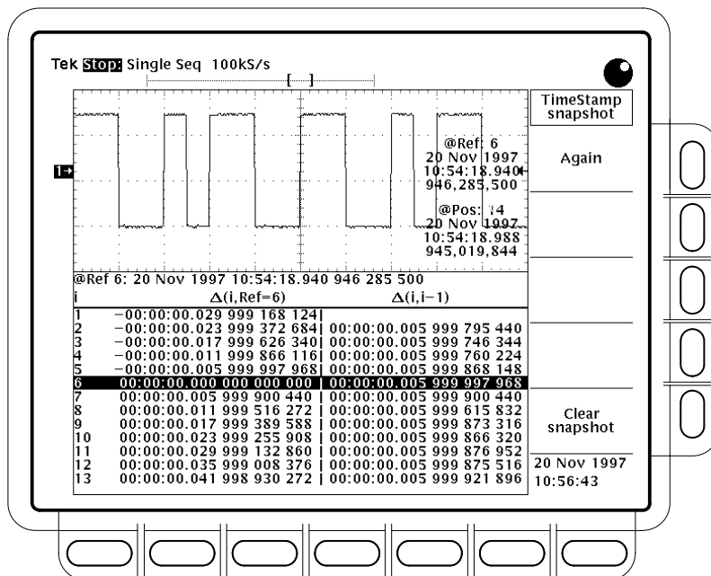
Figure 3–34: Horizontal Menu — FastFrame Snapshot
