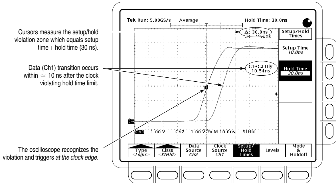
Figure 3–48: Triggering on a Setup/Hold Time Violation
