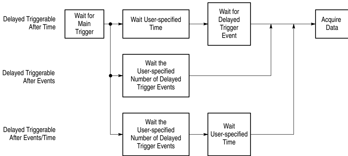
Figure 3–55: Delayed Triggerable
