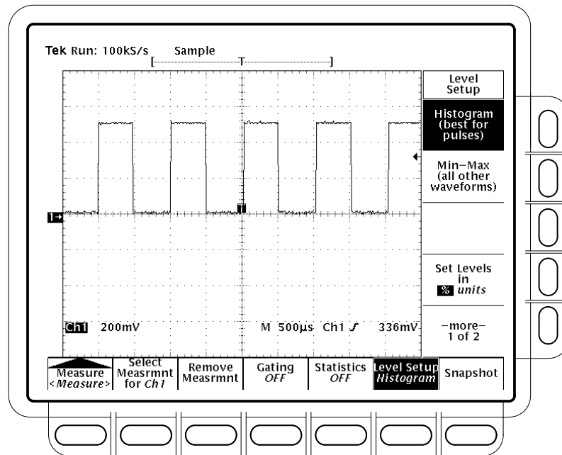
Figure 3–62: Measure Menu — Reference Levels
