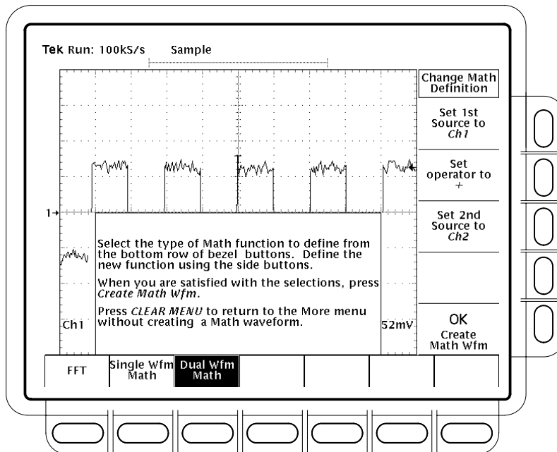
Figure 3–95: Dual Waveform Math Main and Side Menus
