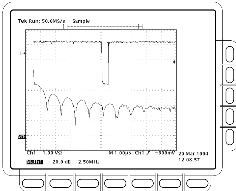
Figure 3-98: FFT Math Waveform in Math1
