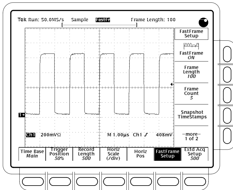
Figure 3–33: Horizontal Menu — FastFrame Setup
