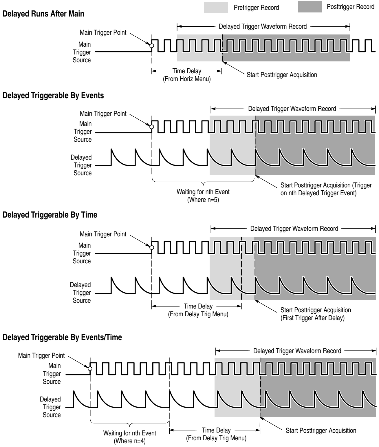
Figure 3-56: How the Delayed Triggers Work
