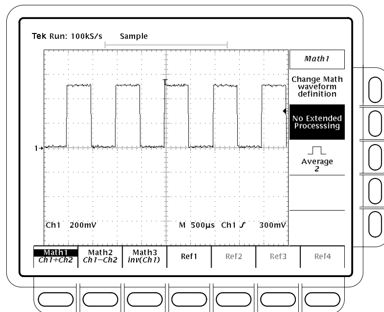
Figure 3–77: More Menu
