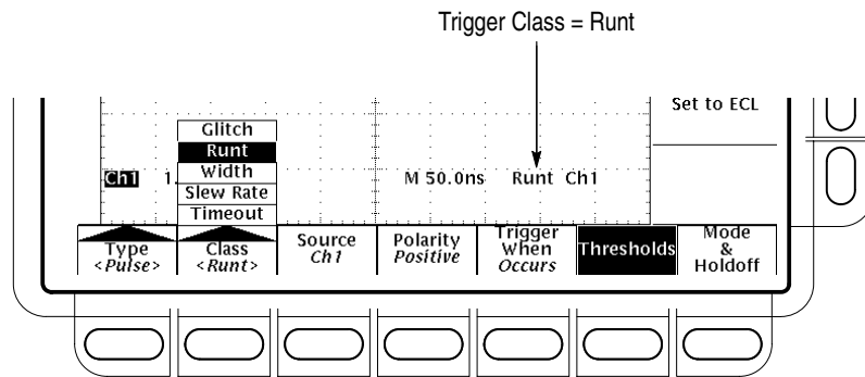
Figure 3–49: Pulse Trigger Readouts
