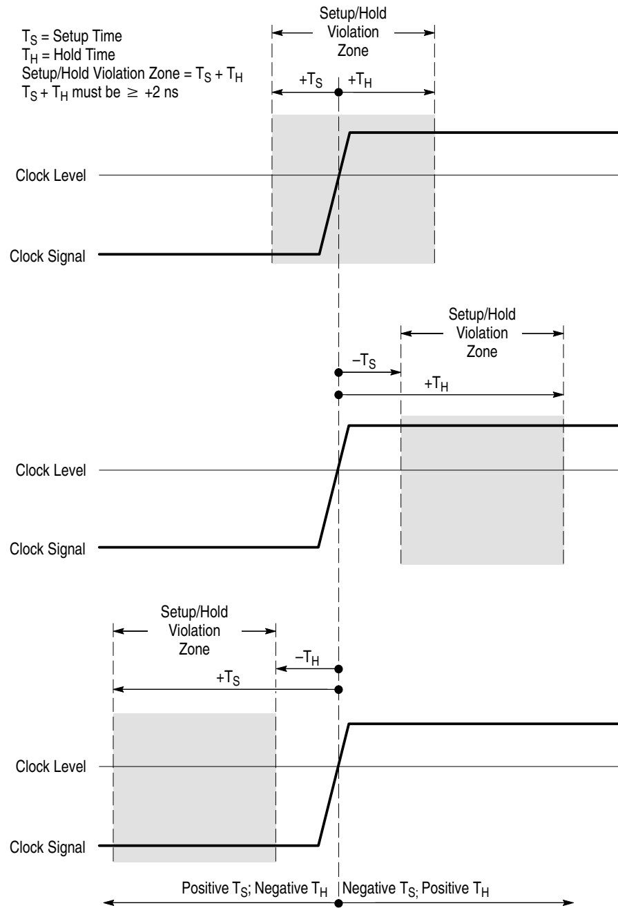
Figure 3-44: Violation Zones for Setup/Hold Triggering
