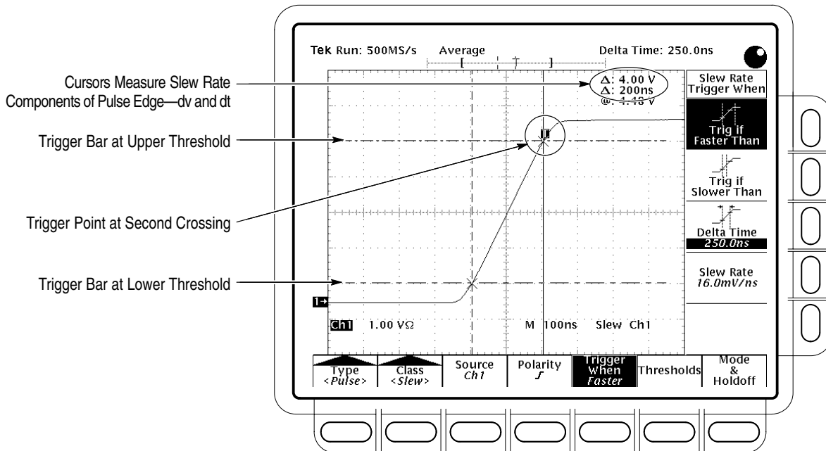
Figure 3–52: Main Trigger Menu — Slew Rate Class
