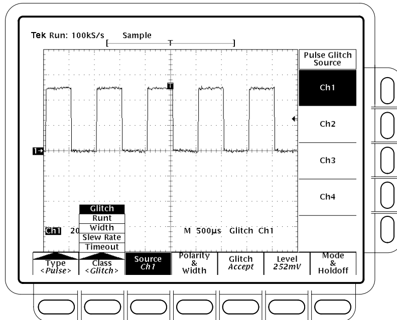
Figure 3–50: Main Trigger Menu — Glitch Class
