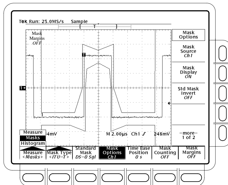
Figure 3–70: Mask menu
