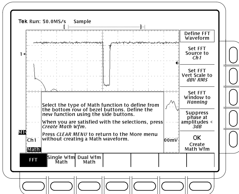
Figure 3–97: Define FFT Waveform Menu
