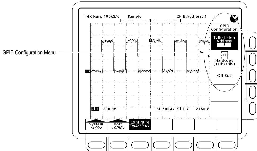
Figure 3–88: Utility Menu
