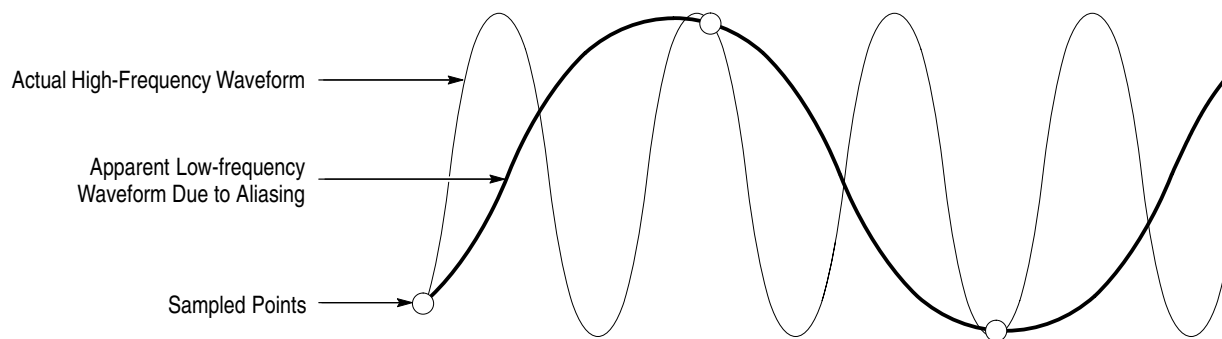
Figure 3-16: Aliasing
