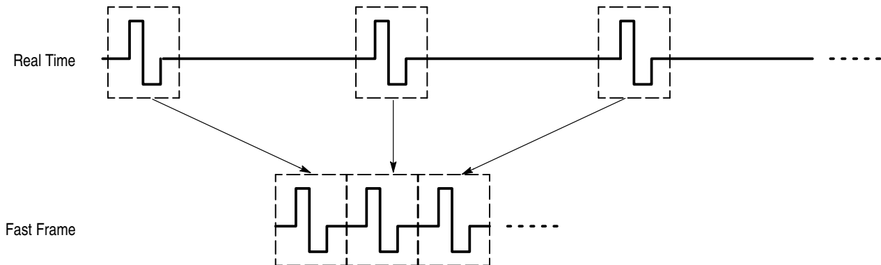
Figure 3–28: Fast Frame
