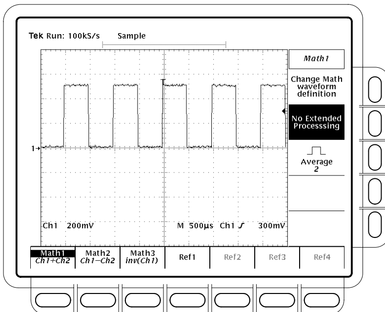
Figure 3–67: More Menu
