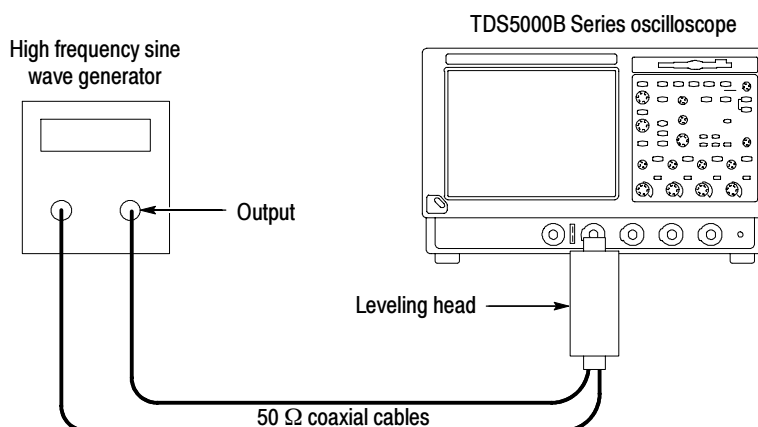
Figure 2-11: Optional initial test hookup
