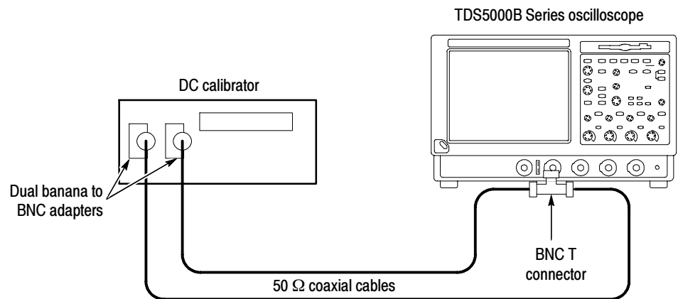
Figure 2-26: Subsequent test hookup
