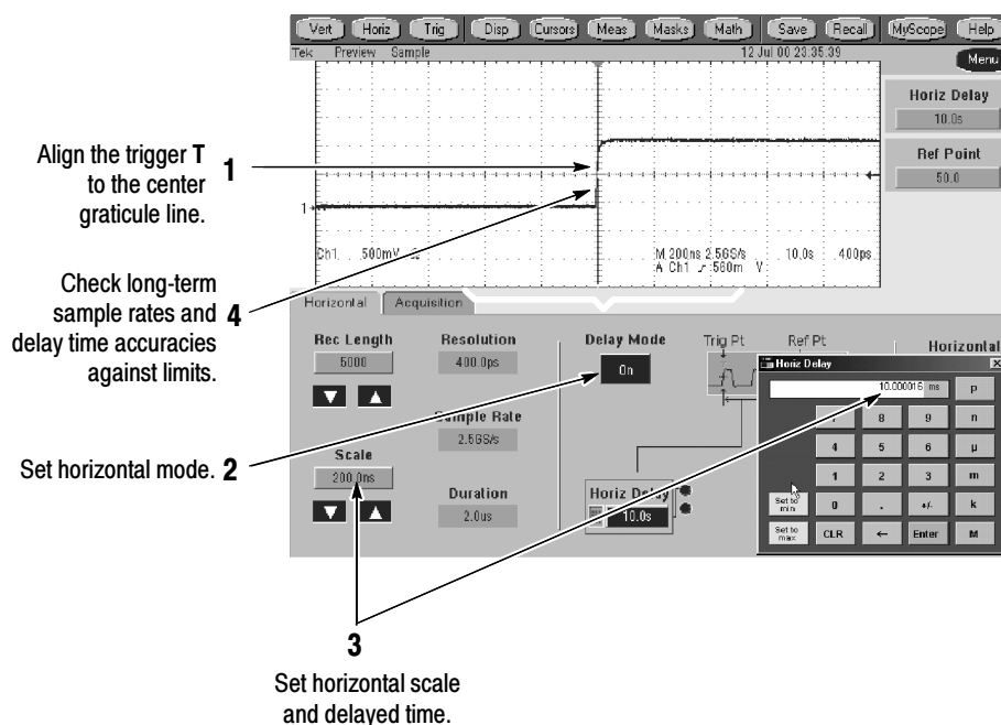
Figure 2-17: Measurement of accuracy - long-term and delay time
