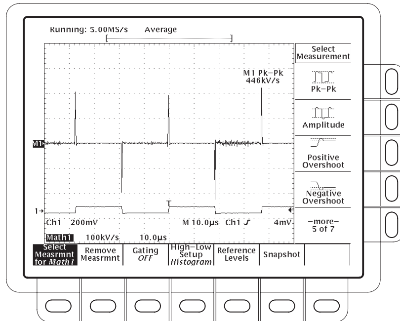
Figure 3-74: Peak-Peak Amplitude Measurement of a Derivative Waveform
