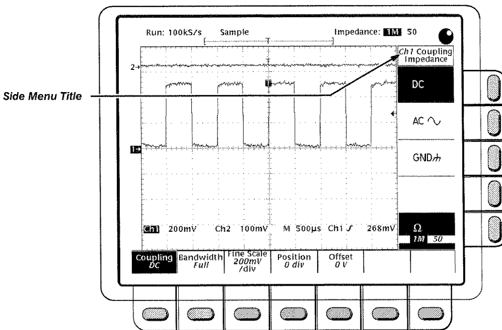
Figure 1-16: The Menus After Changing Channels
