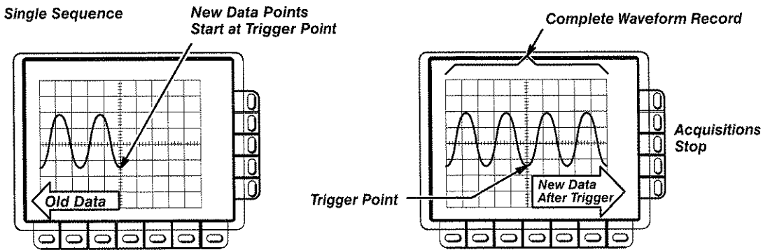
Figure 3-44: Roll Mode (500 Point Record Length)
