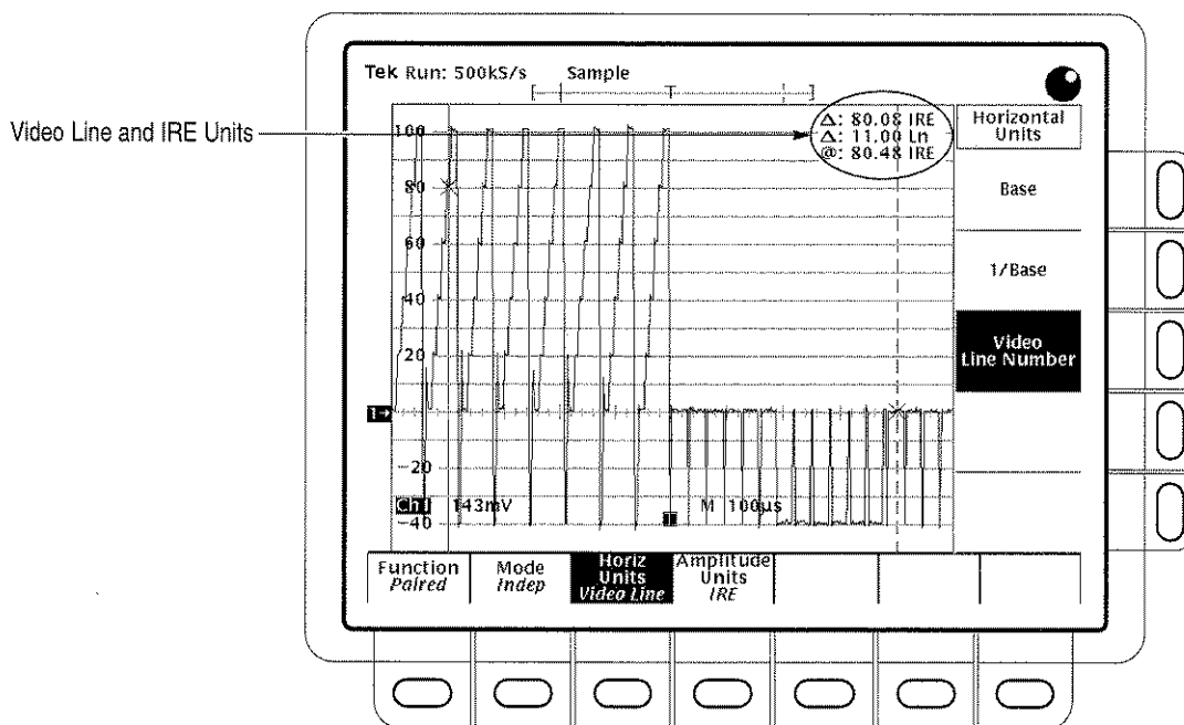
Figure 3–57: Video Line and IRE Units
