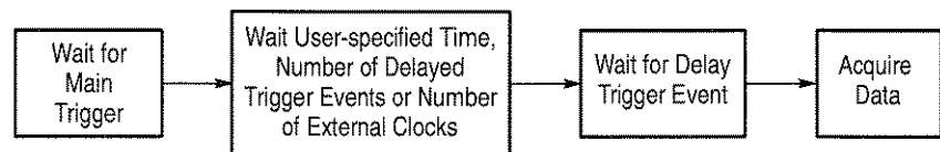
Figure 3-6: Delayed Triggerable
