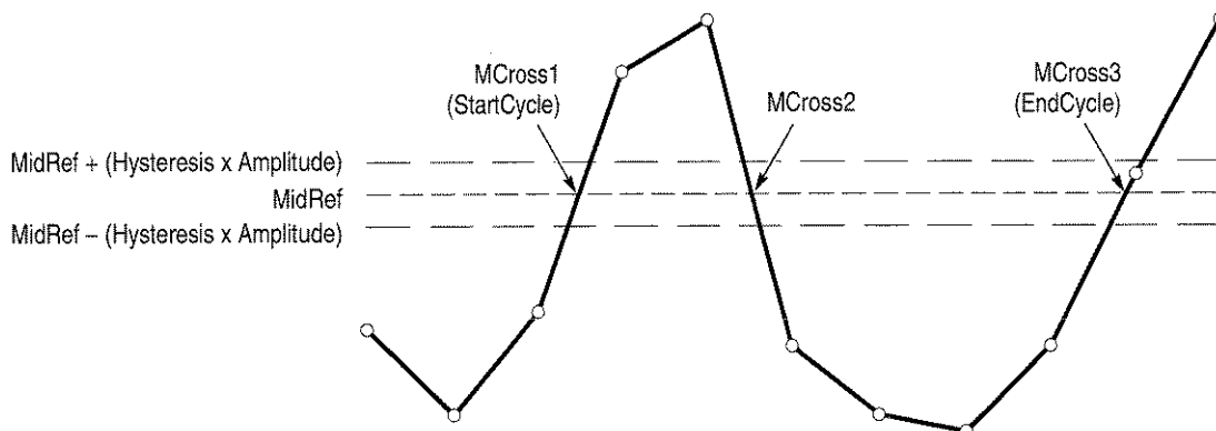
Figure C-1: MCross Calculations
