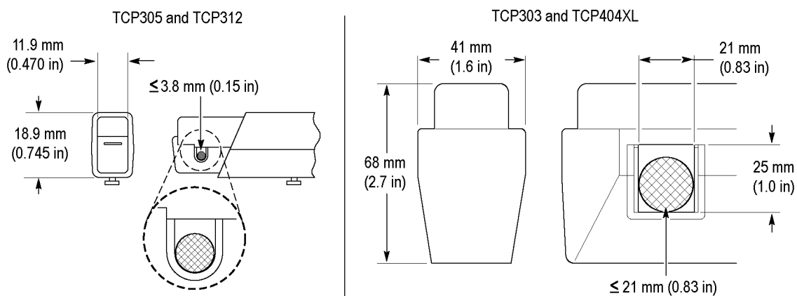
Figure 27: Probe jaw dimensions (nominal)
