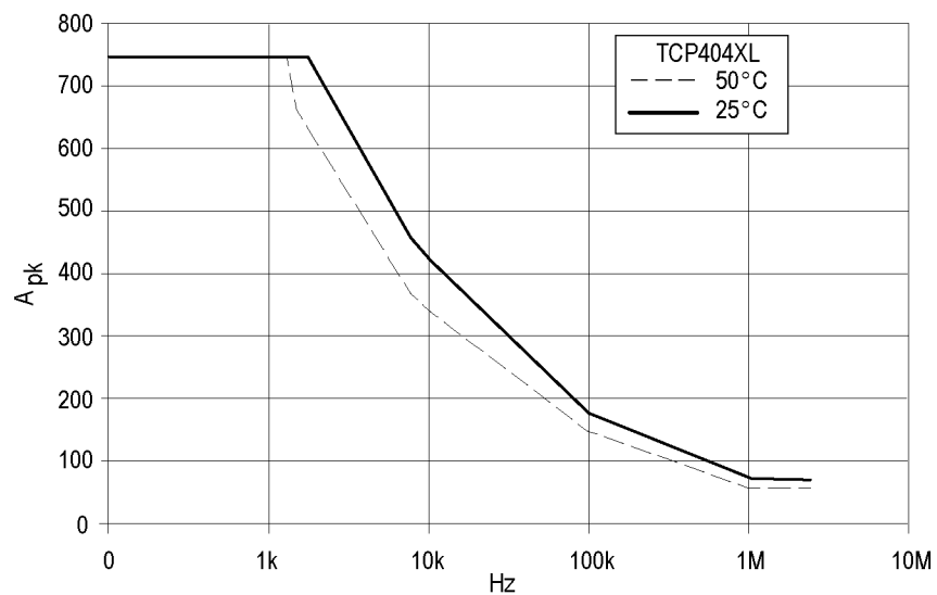
Figure 31: Frequency derating-TCP404XL
