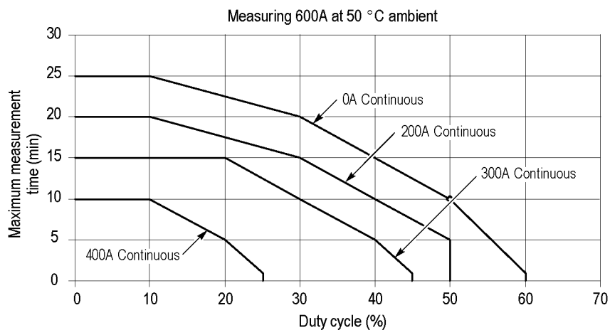
Figure 35: Measuring 600A noncontinuous at 50 °C ambient temperature
