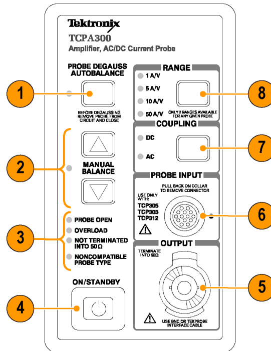
Figure 9: The TPCA300 front panel
