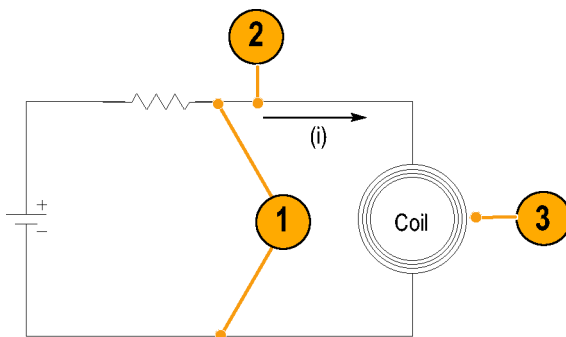
Figure 23: Measuring the number of turns in a coil
