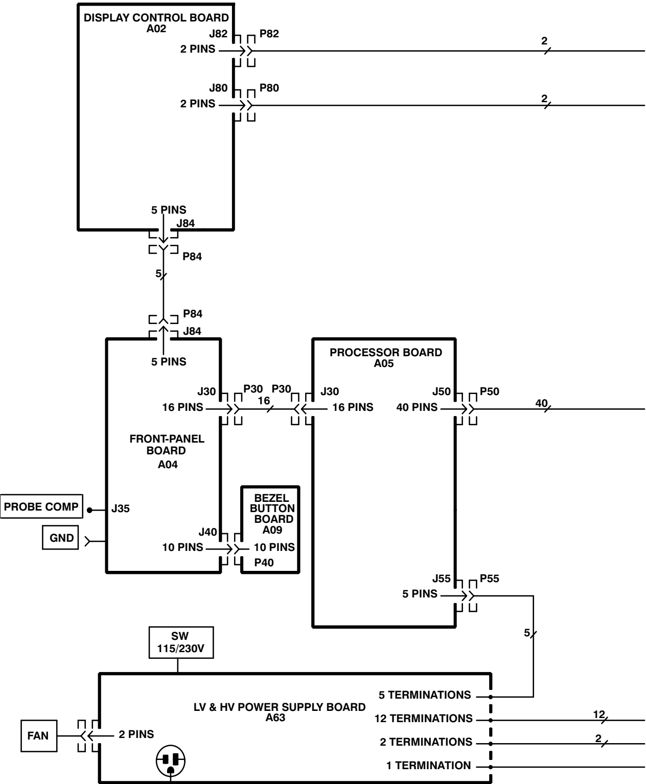
Figure 3-1: Block Diagram
