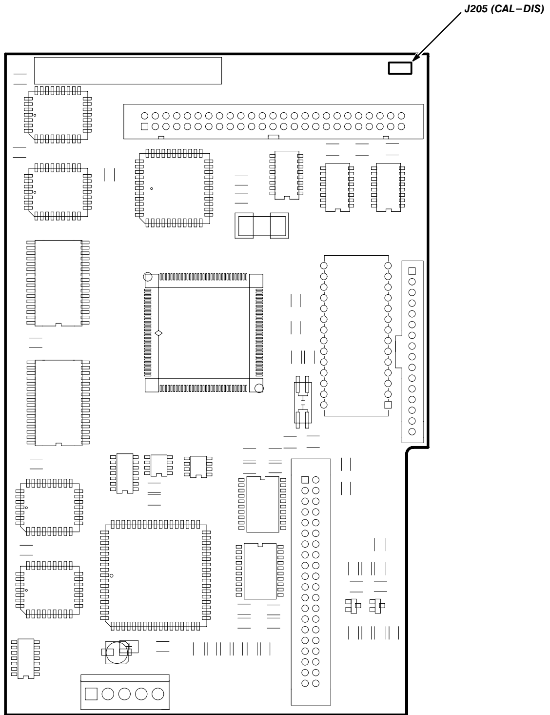
Figure 5-17: Location of J205 (CAL-DIS) on the CPU Board
