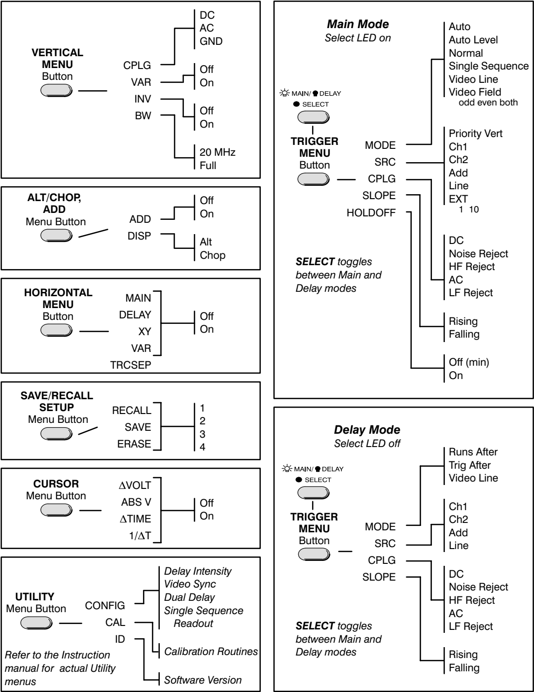
Figure 2-8: Menu Map
