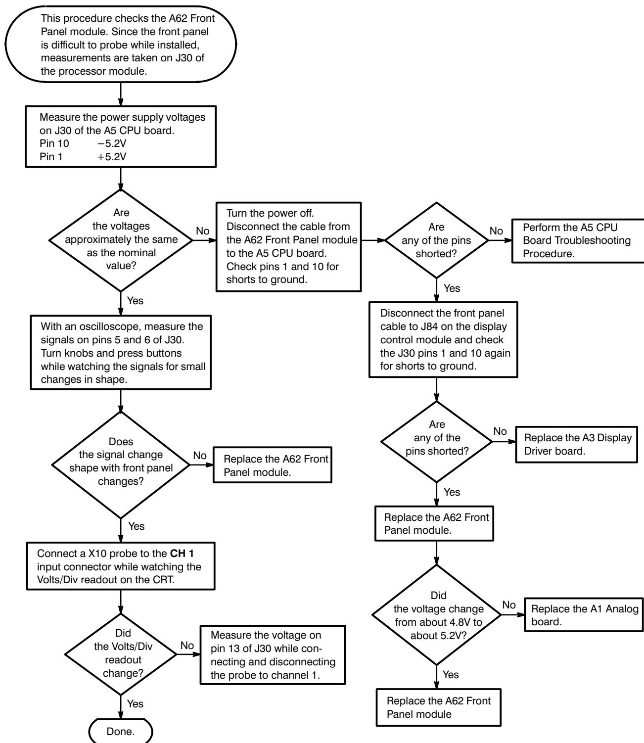
Figure 6-27: A62 Front Panel module Troubleshooting Procedure
