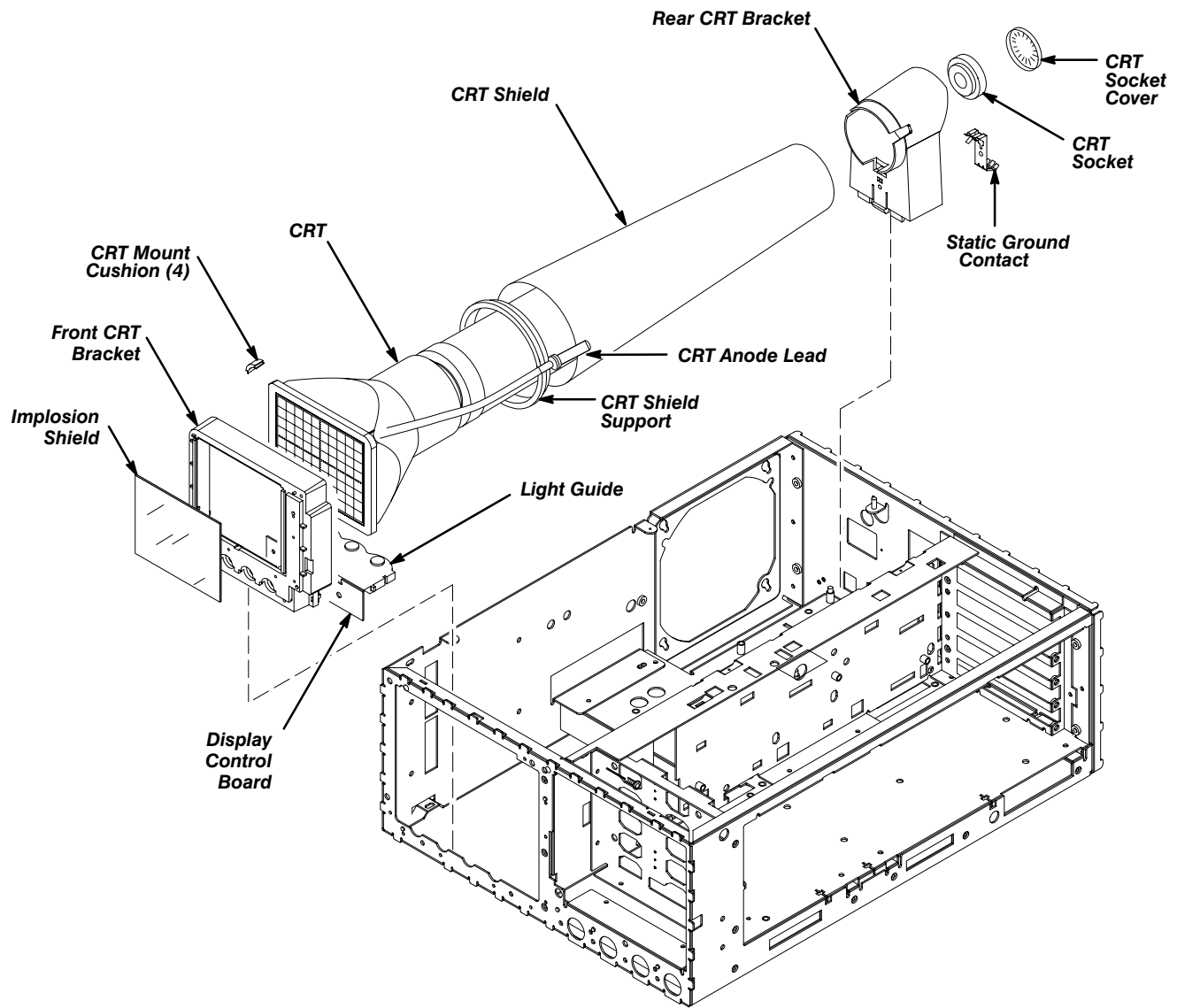
Figure 6-19: CRT Removal
