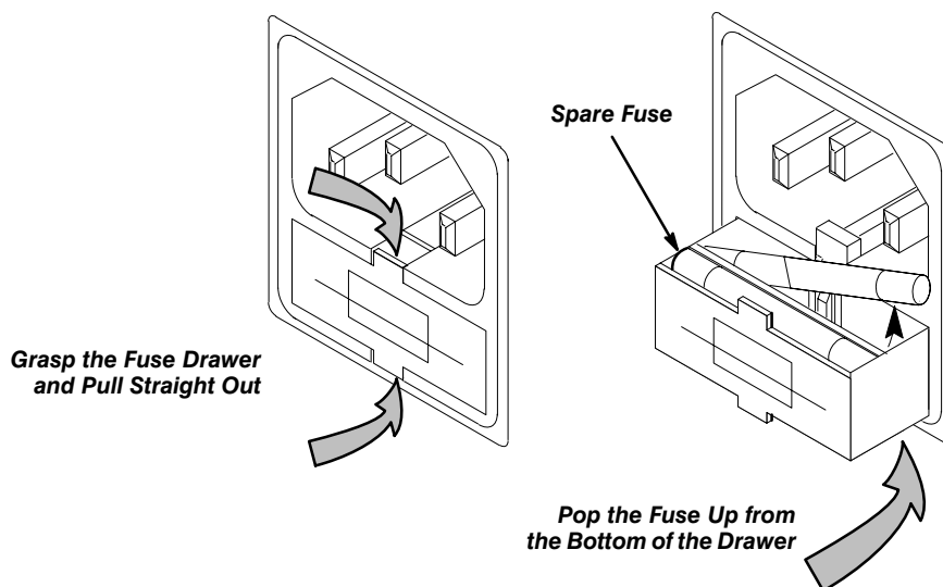
Figure 2-2: Fuse Compartment
