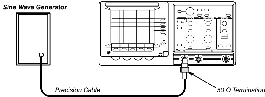
Figure 4-8: Bandwidth Test Setup
