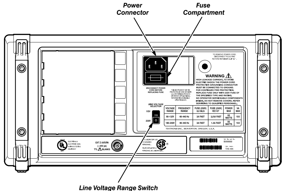
Figure 2-1: Rear Panel
