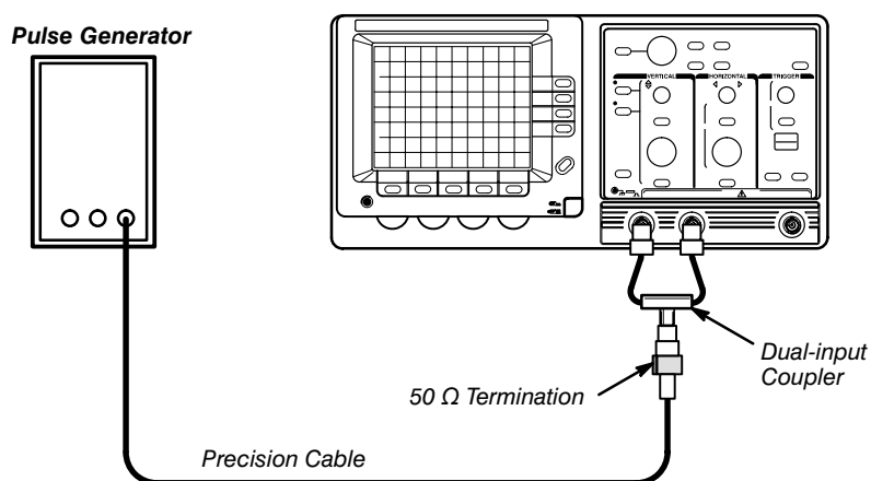
Figure 5-13: Attenuator Compensation Test Setup
