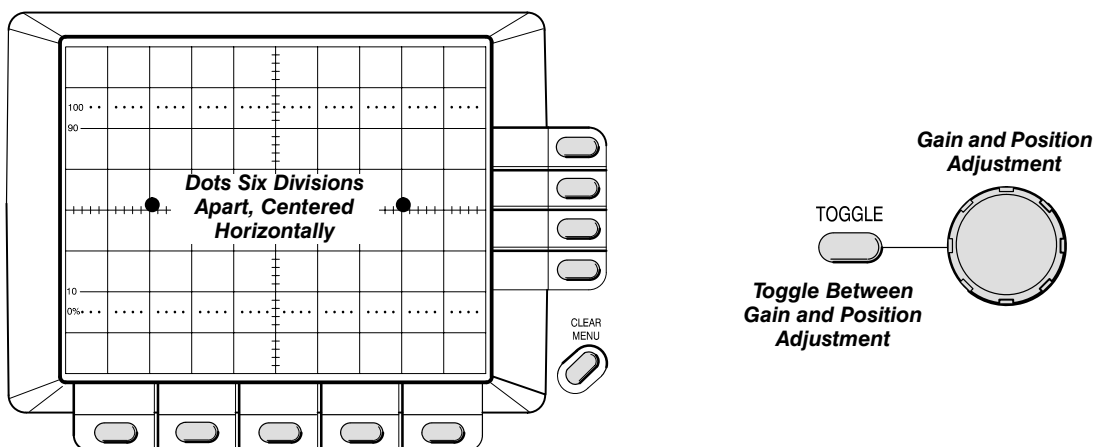
Figure 5-10: Vertical Adjustments
