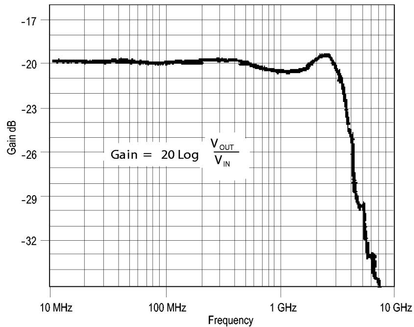
Figure 2: Typical bandwidth
