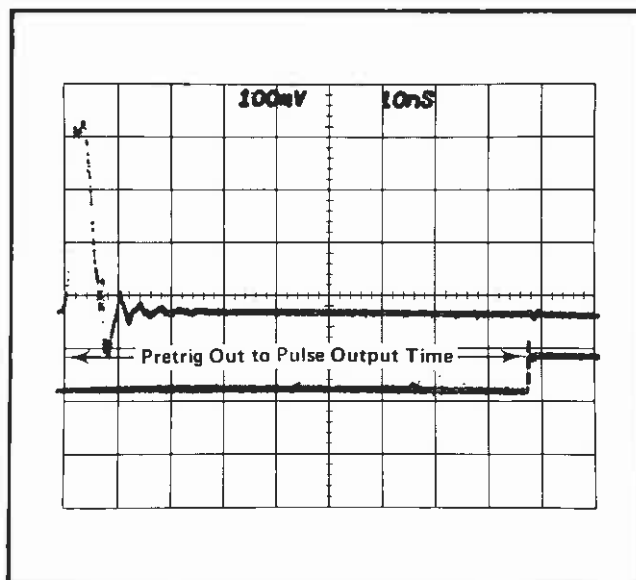
Fig. 5-3. Double exposure photo showing the PRETRIG OUT to PULSE OUTPUT time interval.
