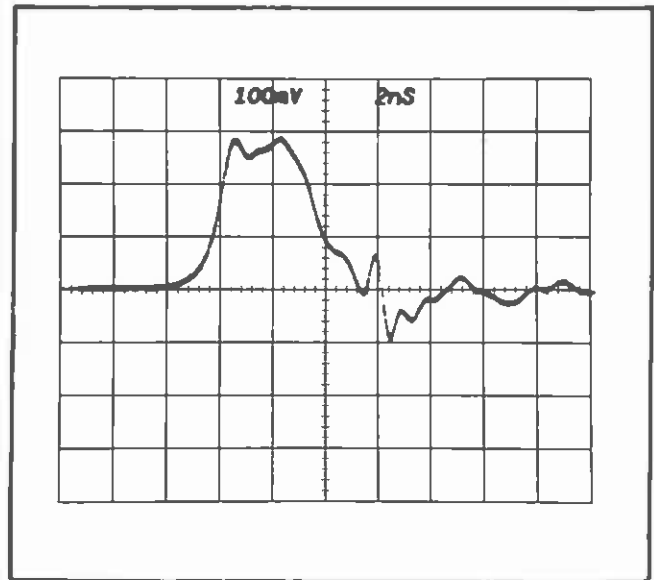
Fig. 5-1. Pretrigger Out.
