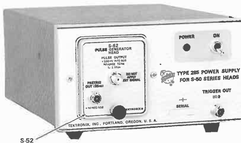
(C) Installed in Type 285 Power Supply Compartment
