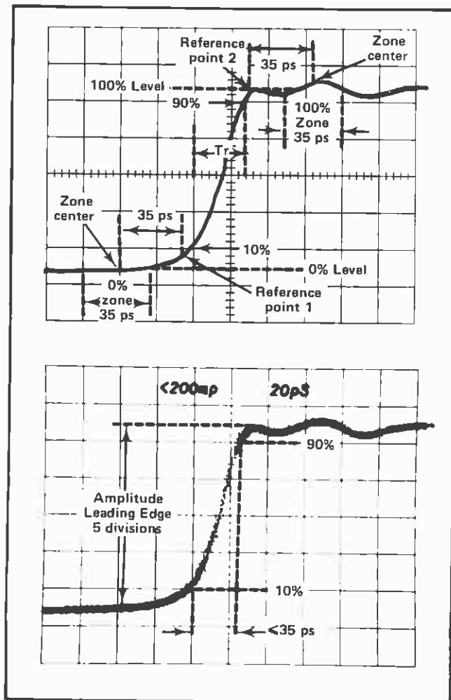
Fig. 5-7. Risettime measurement ( T_r ) information (upper) and typical risetime display (lower). Note that Reference point 1 and 2 are selected at the corners where the rate of change of the slope is maximum (where the radius of curvature is least).
