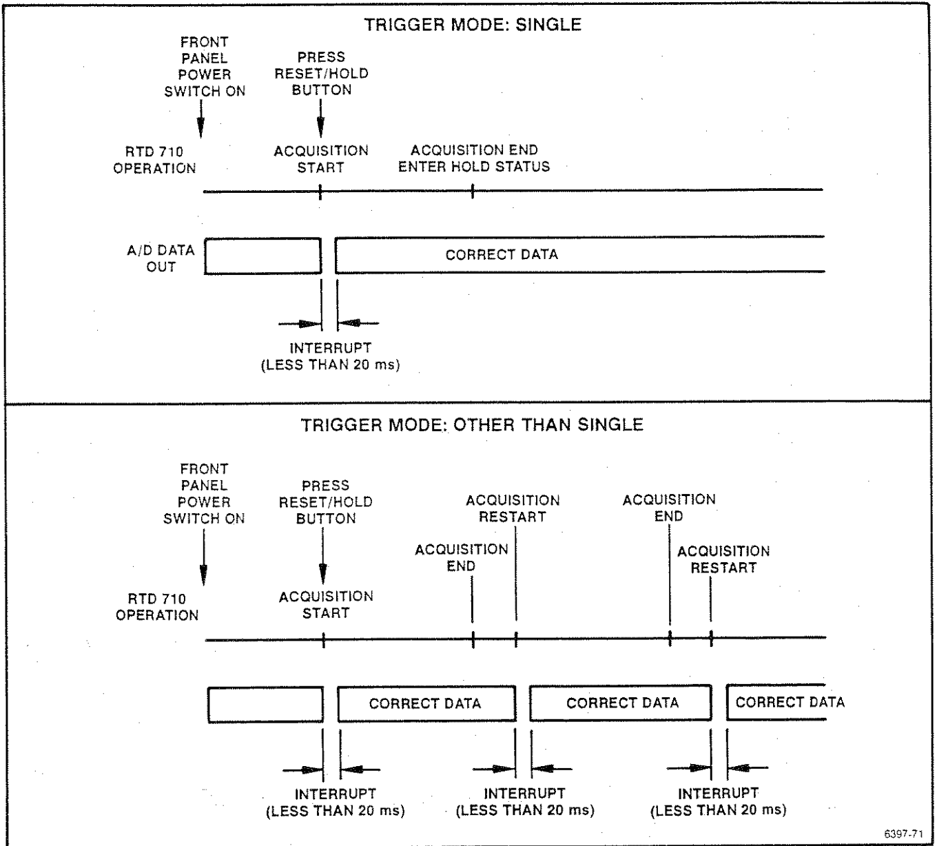
Fig. 4-6. A/D output operation.
