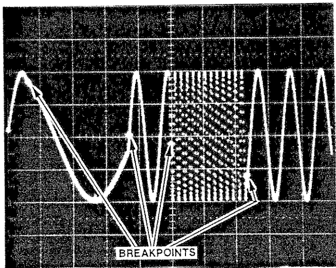
Fig. 3-33. Breakpoint waveform with post-trigger.
