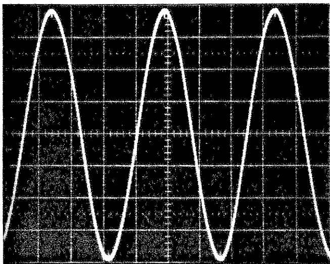
Fig. 3-11. Input range setting correct: Input Signal = \pm 0.5 V; RANGE = \pm 500 mV.
