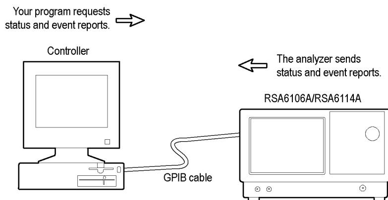
Figure 1-3: Event-driven program
