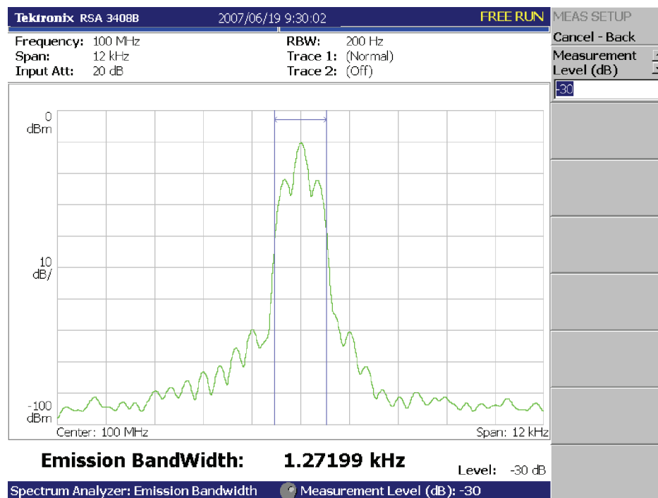
Figure 3-13: EBW measurement
