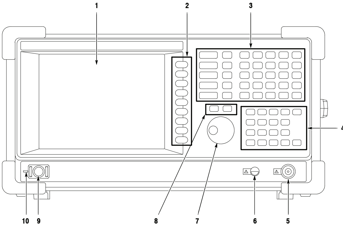
Figure 2- 1: Front panel
