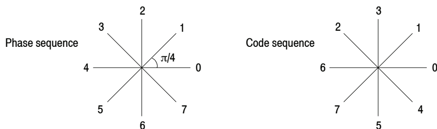
Figure 3- 150: D8PSK symbol value
