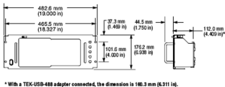
Figure 1: RM2000B Rackmount assembly
