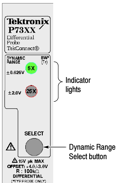
Figure 2: Probe (front)
