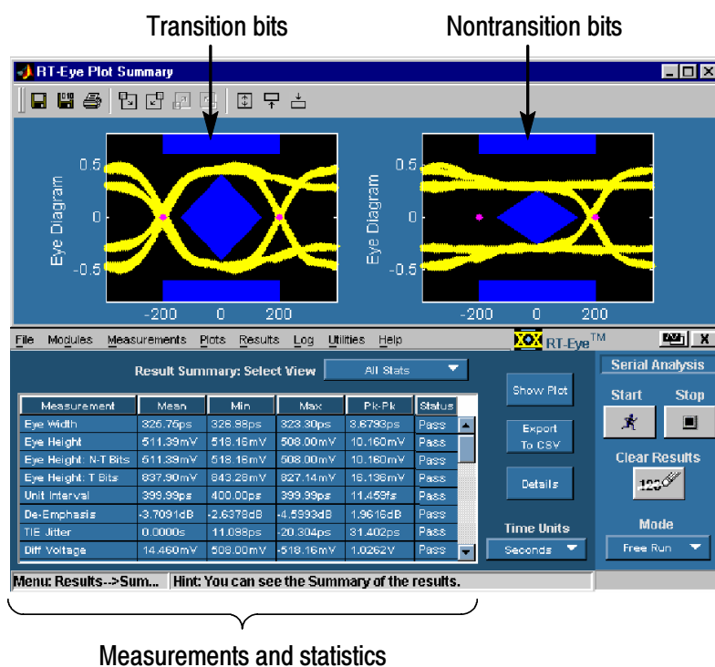
Figure 23: RT-Eye application
