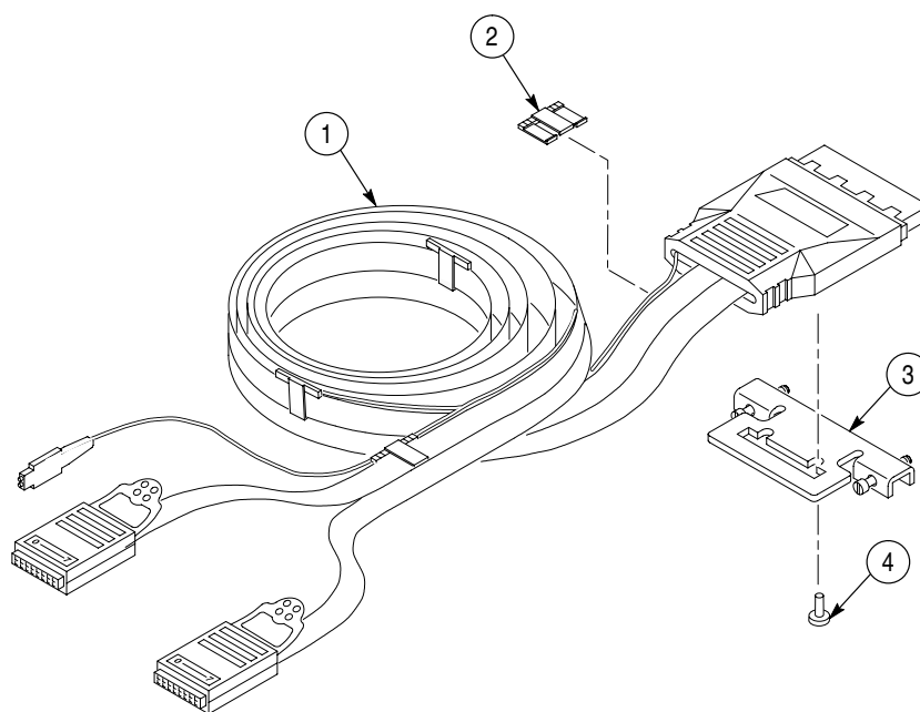
Figure 19: P6418 Probe exploded view
