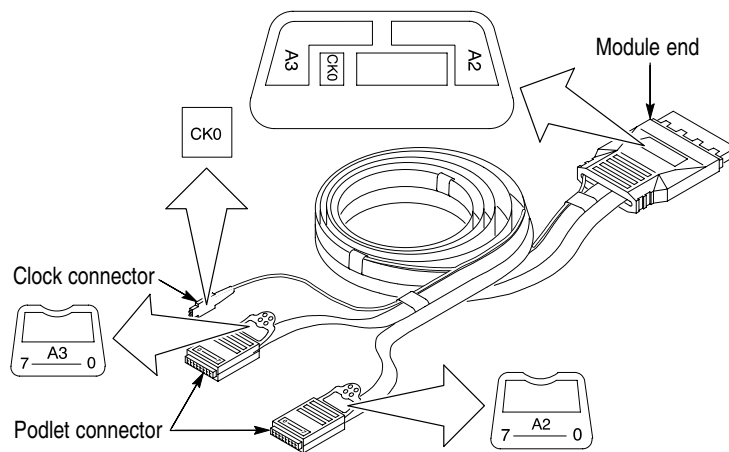
P6418 Probe
