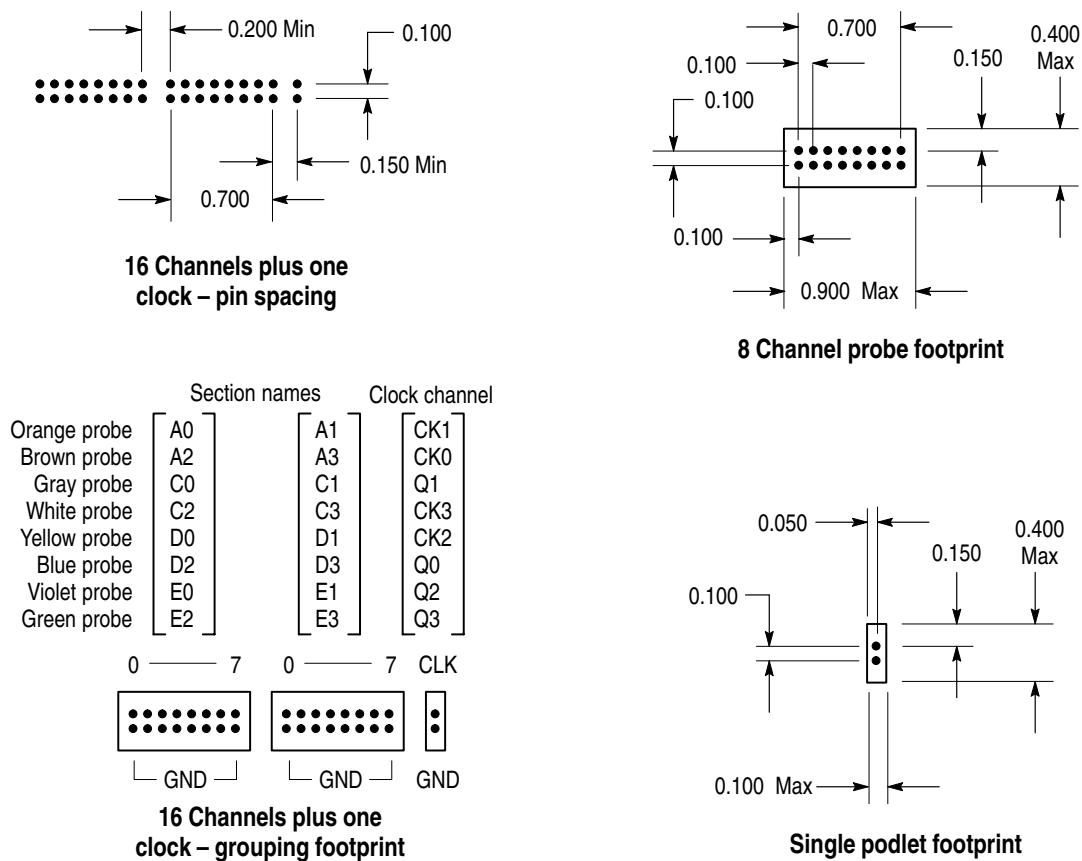
Figure 5: Probe footprints
