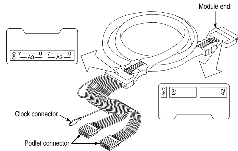
P6417 Probe
