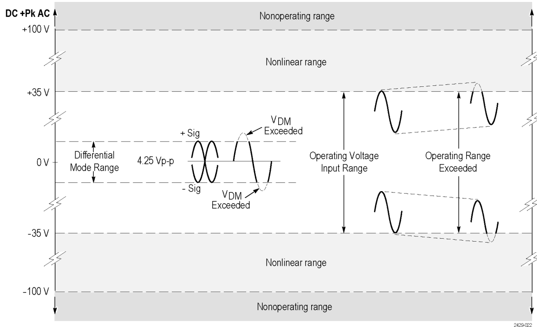
Figure 2: Input voltage limits with no DC offset, 4.25 V (±5) range
