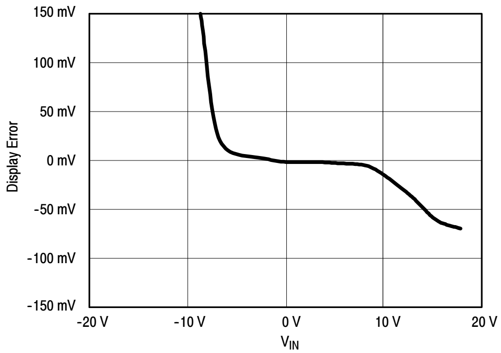
Figure 2: Typical Linearity Error vs. V IN
