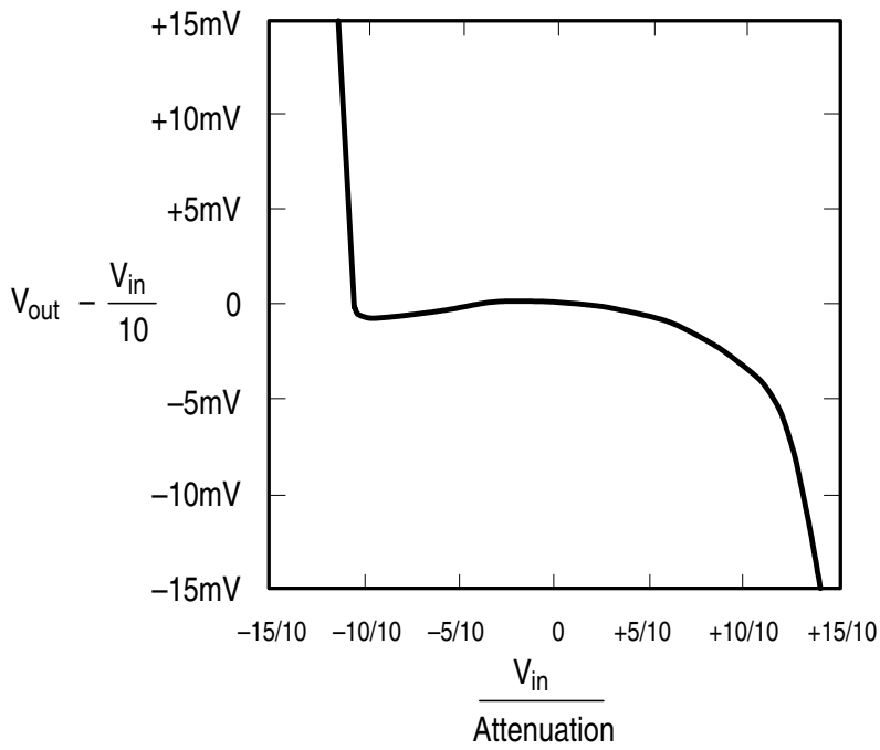
Figure 3-3: Linearity error vs output voltage
