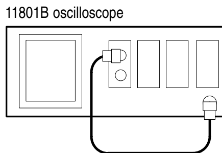
Figure 4–1: Attenuation test setup part 1
