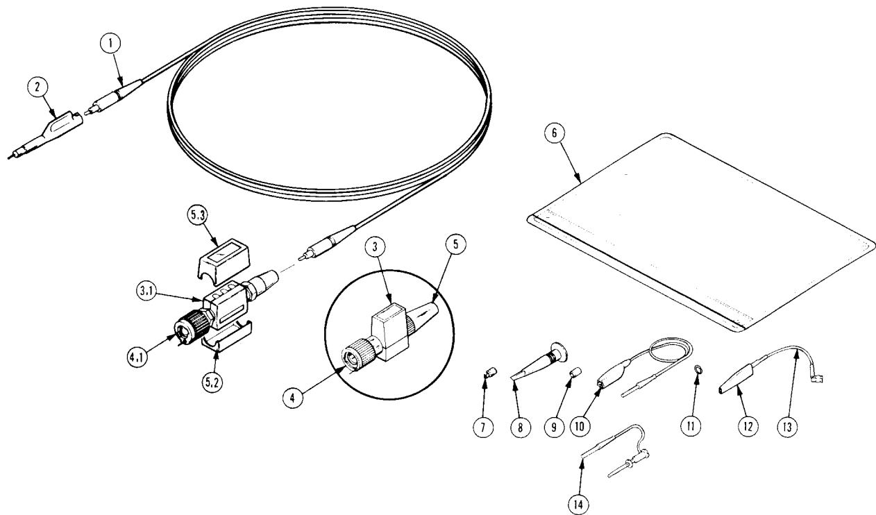
Figure 6-1. Exploded View
