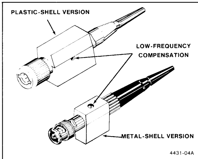
Figure 4-1. Low frequency adjustment.
