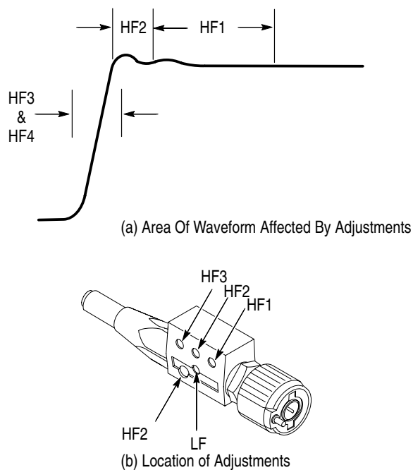
Figure 1: HF Compensation
