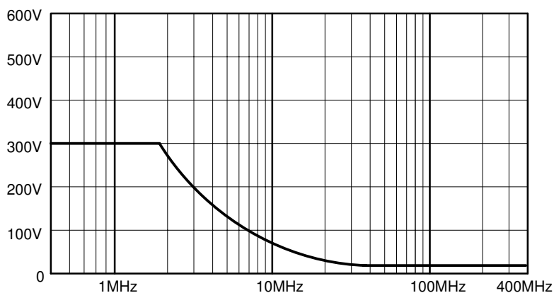
Figure 2: Maximum Working Voltage Derating Curve ( V_{RMS} )
