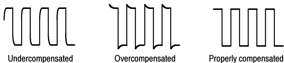
Figure 1: Probe compensation waveforms
