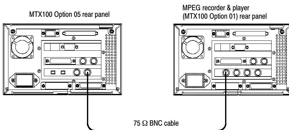
Figure 4-22: ASI interface Record operation test
