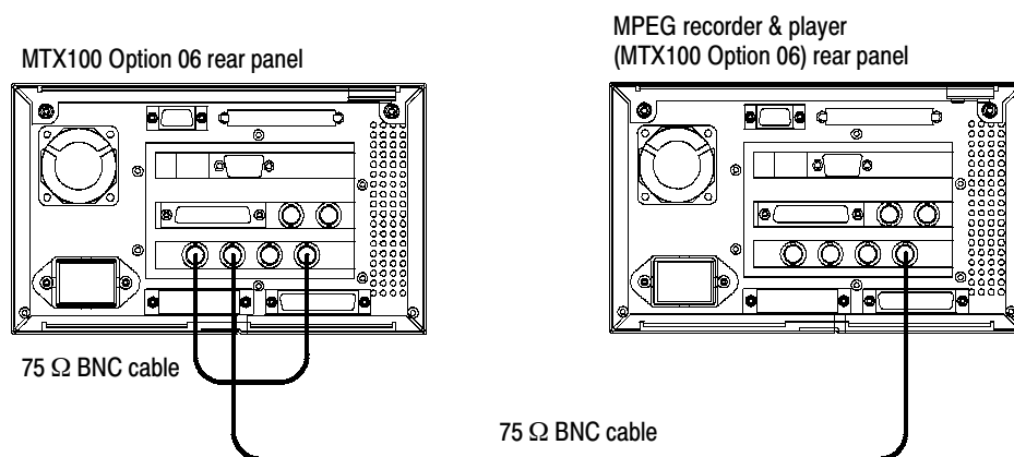
Figure 4-29: SMPTE310M/8VSB interface test
