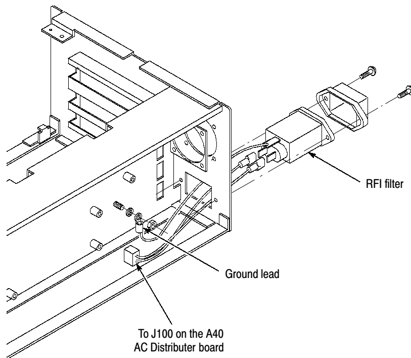
Figure 6-15: RFI filter removal
