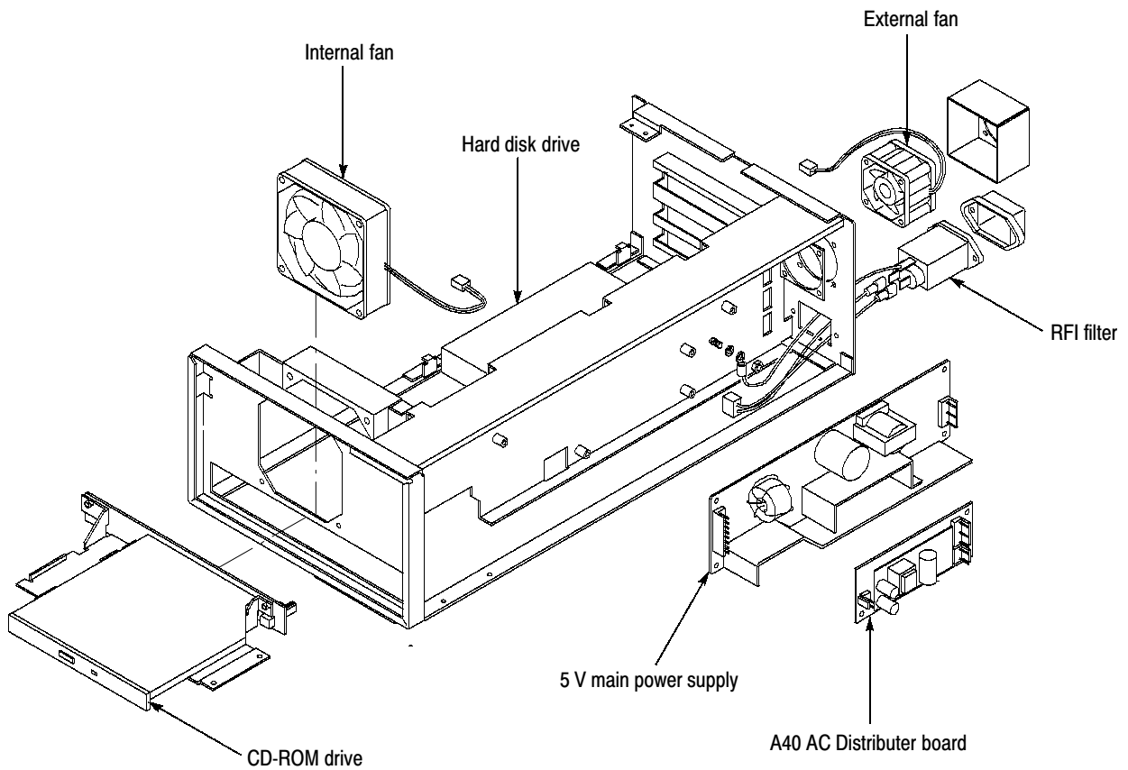
Figure 6-4: Internal modules
