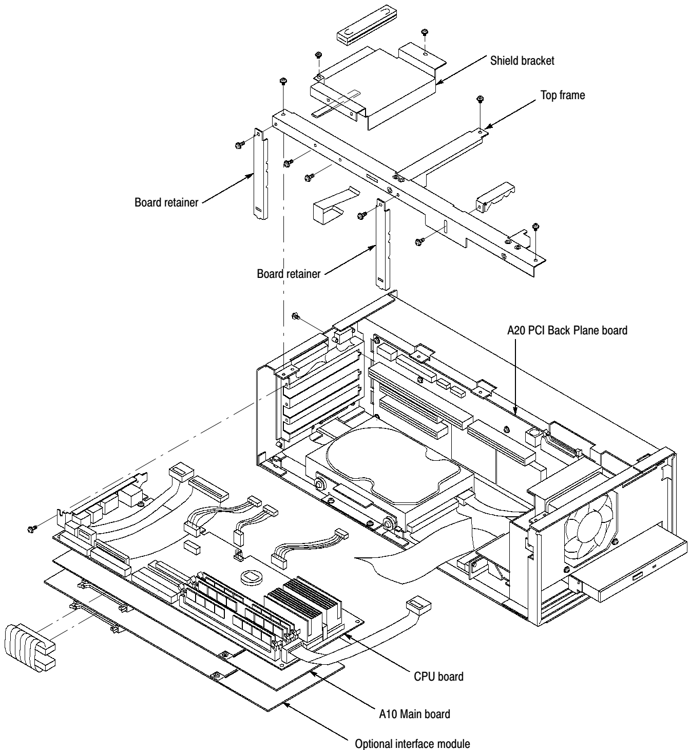
Figure 6-10: CPU board, A10 Main board, interface module, and A20 PCI Back Plane board removal
