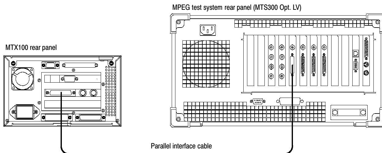
Figure 4-5: Second equipment connection for verifying the SPI interface
