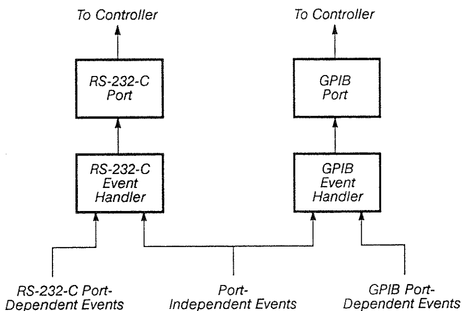
Remote Interface Status Reporting System Block Diagram
